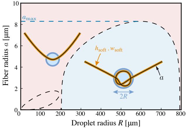
Figure 7: Graphical representation of the inequality (12) (blue dashed line) for a silicone oil drop ( \gamma = 21 mN/m, \rho g = 9600 N/m 3 ) sitting on a composite fiber composed of a core fiber of radius a and Young's modulus E = 1 GPa in this example, and a soft auxiliary PVS beam ( w_{\text{soft}} = 190 \mu\text{m} , h_{\text{soft}} = 65 \mu\text{m} , E_{\text{soft}} = 200 kPa). The small tongue near the origin corresponds to the one shown in figure 4, for a silicone oil droplet sitting on a bare fiber. The soft auxiliary artifact allows to achieve coiling for much thicker fibers (larger a ). The largest theoretical coilable fiber has a radius a_{\text{max}} explicit in equation (13).
