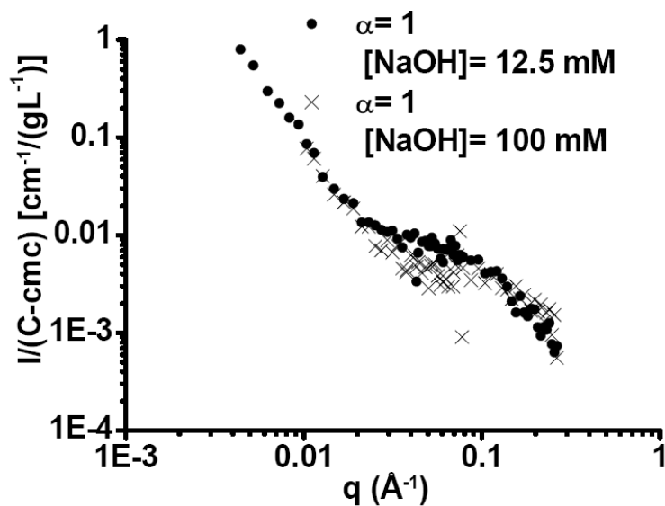
Figure 8 –SANS experiments performed on two SL solutions at \alpha=1 but different NaOH concentrations. Data on the [\text{NaOH}]=12.5 mM (pH= 11) system (full circles) were completed with ultra-low angle experiments ( q < 8.38 \cdot 10^{-3} \text{ \AA}^{-1} ) to confirm the increase of I(q) .
