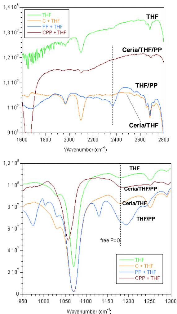
Figure S1 - FTIR spectrum of 5-phenyl-phosphonic acid (PPA) functionalized ceria nanoparticles in THF. For completion, THF, Ceria/THF and THF/PP spectra are shown. The functionalization of the nanoparticles is followed by FTIR spectroscopy. Disappearing of FTIR bands of free P-O vibration in the 2200-2300 \text{cm}^{-1} region and lack of free P=O band in the 1200 \text{cm}^{-1} region suggest a tridentate binding of phosphonate group. [see a) Botelho do Rego et al (2005) Langmuir 21:8765; b) Bae et al (2004) J Phys Chem B 108:14093; c) Podstawka et al (2005) Surf Sci 599:207; d) Lin-Vien et al (1991) The handbook of IR and Raman characteristic frequencies of organic molecules, Academic Press, San Diego]
