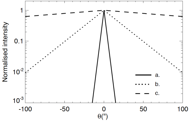
Fig. 3. Intrinsic dust profiles (see Eq. (17)) for scenarios a. , b. and c. listed in Table 1, corresponding to characteristic scale heights of z_d = 0.1 , 1 and 10 kpc, respectively. These profiles are then convolved with Herschel PSFs to simulate an edge-on galaxy observed in different bands.
