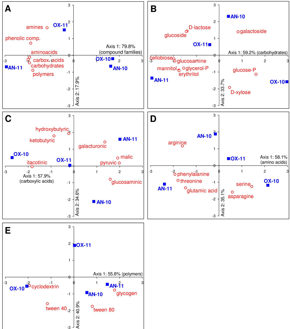
Fig 8. Principal component analysis (PCA) of Biolog ECO plates community metabolic potential. AWCD after 96 h incubation was used as input data. Samples are represented by blue squares, with OX and AN for oxic and anoxic conditions respectively, with sampling year provided. PCA were performed for compound merged (A) in families, or molecules within a chemical group: (B) carbohydrates, (C) carboxylic acids, (D) amino acids, and (E) polymers.
