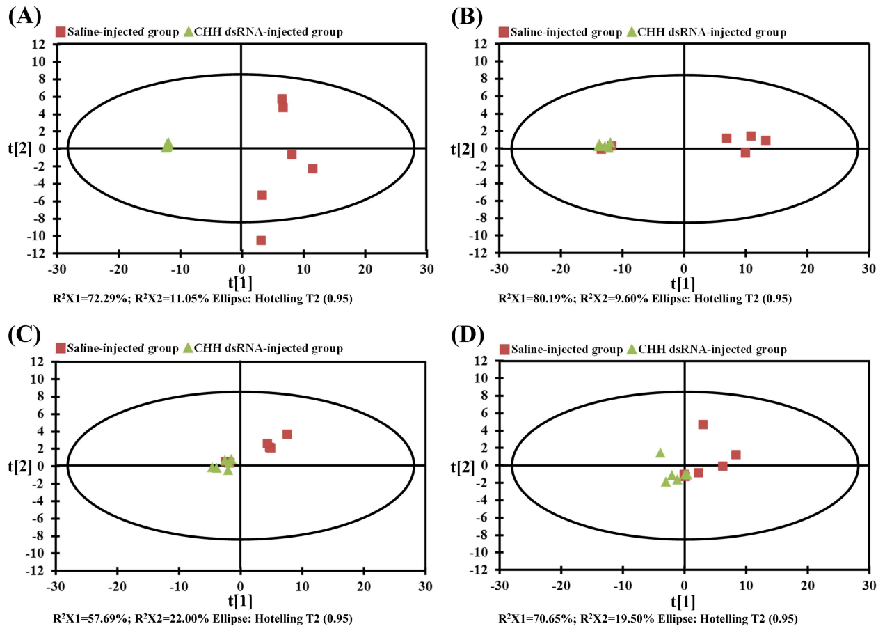
Fig 4. Principal component analysis plot of tissue samples of the crayfish Procambarus clarkii showing differential metabolic profiles between saline-injected and CHH dsRNA-injected groups. A, B: the muscle at 24 and 48 hpi, respectively; C, D: the hepatopancreas at 24 and 48 hpi, respectively. Triangle: CHH dsRNA injected group; Square: saline-injected group. Each symbol represents the metabolome of a single sample along two principal components.
