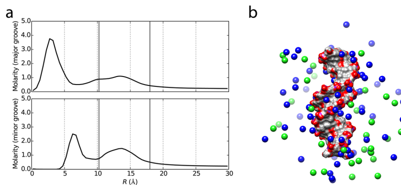
Figure 13. (a) Radial distribution of K^+ ions along the distance to the DNA helical axis, averaged over a series of microsecond simulations of different tetranucleotides at physiological ion concentration, in the major (upper panel) and minor (lower panel) grooves (Reproduced with permission from ref 278. Copyright 2015.). (b) Distribution of K^+ (blue) and Cl^- (green) ions around DNA, where the oxygen and phosphorus atoms are highlighted in red and purple, from a snapshot of the simulation described in ref 278 (Image courtesy of R. Lavery).
