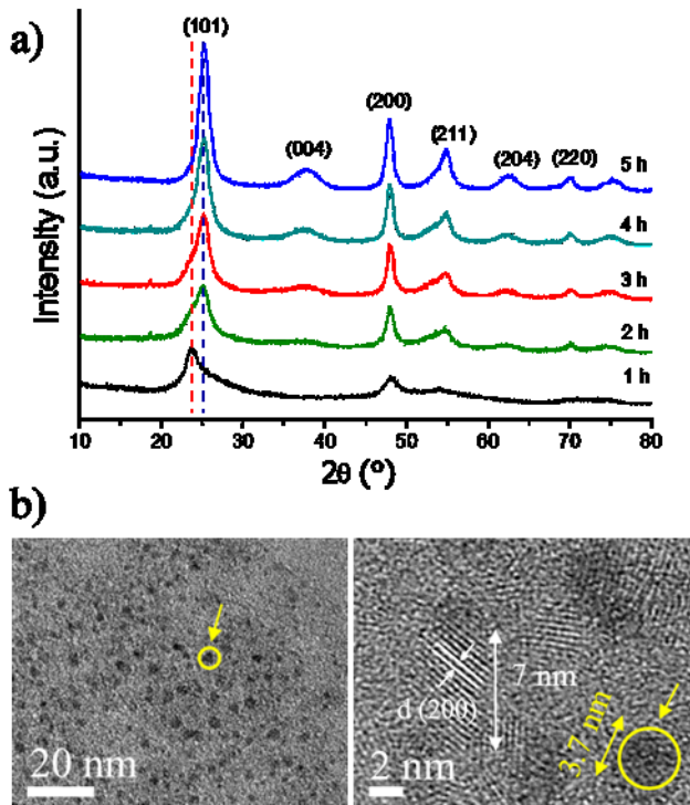
Figure 1. (a) XRD patterns of the samples synthesized within the first 5 hours. (hkl) planes of anatase are indicated. Red and blue dashed lines correspond to the (100) and (101) planes of \text{TiOF}_2 and anatase, respectively. (b) HRTEM images of the sample obtained after 1 h of reaction.
