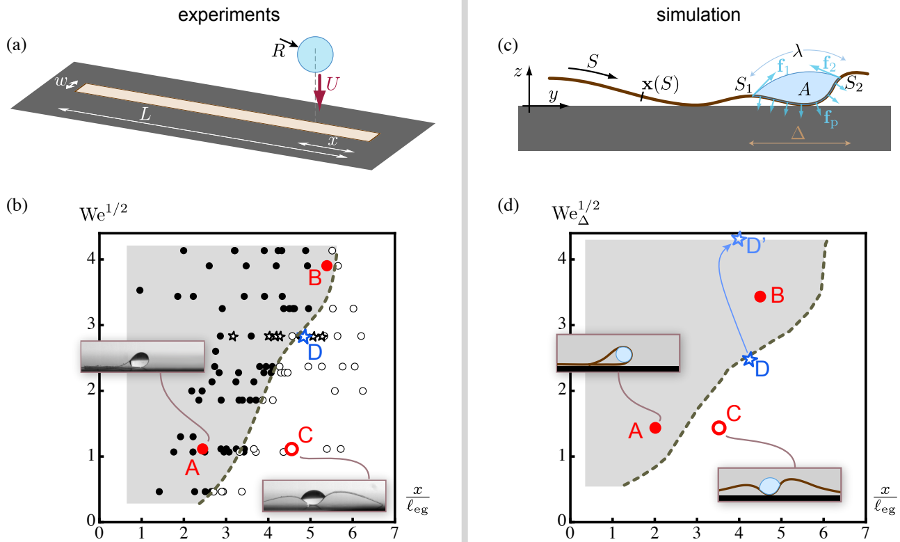
Figure 3. Comparison of experiments (a,b) and simulations (c,d) in a 2D geometry. (a) In these experiments, a drop impacts a long, thin polymer strip laying down on a substrate, at a variable distance x from its end, and with variable impact velocity U . Strip dimensions are L = 5 cm and w = 2 mm, and drop radius is R = 1.55 mm. (b) Phase diagram showing the outcome of the experiment: non-encapsulated drop (open circles), encapsulated drop (filled dots), or encapsulated drop with the help of a secondary drop obtained by pinch-off (stars). (c) Numerical model of a 2D dynamic Elastica coupled with a quasi-static, incompressible fluid with surface tension. (d) Phase diagram for the Elastica model. In (b,d), typical final shapes are shown in inset. The time sequences of a few selected experiments, labelled A, B, C and D here, are compared in figures 4 and 5. During the simulation run labelled D in (d), the impact parameters are changed to account for the capture of a secondary drop, as shown by the light blue arrow.
