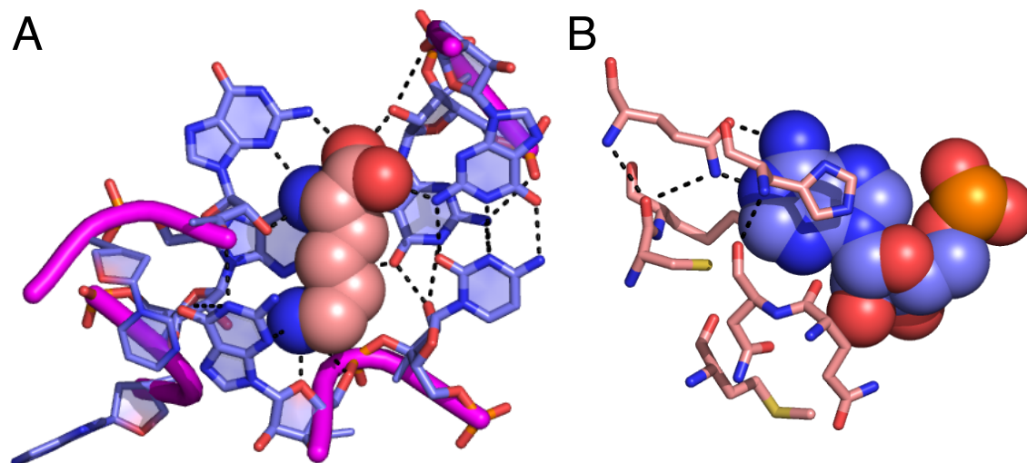
Figure 4.1: RNA/amino acid and nucleotide/protein interactions as a potential relict of the primordial genetic code. (A) Interaction between a lysine amino acid and a riboswitch. The amino acid is shown using an atomic CPK (Corey–Pauling–Koltun) model and the nucleotides from the RNA riboswitch by a stick model (the RNA chain is shown by a purple ribbon). The charged amino acid interacts simultaneously with several nucleotide residues of the RNA. Hydrogen bond contacts are indicated by dashed lines (PDB ID: 3D0U). (B) Interaction between a nucleotide residue (adenosine) from an RNA chain and a human protein (PUMILIO1). The nucleotide is shown using an atomic CPK model and the surrounding protein residues by a stick model. The nucleotide residue interacts simultaneously with several amino-acid residues (PDB ID: 1M8W).
