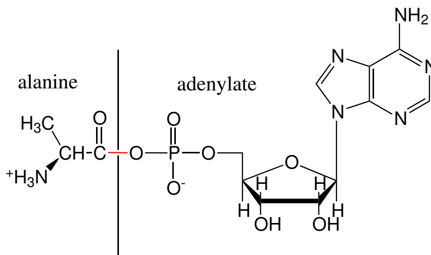
Figure 3.1: Chemical structure of alanine-adenylate. The energy-rich bond between the carboxyl, and the phosphate group is indicated in red.
