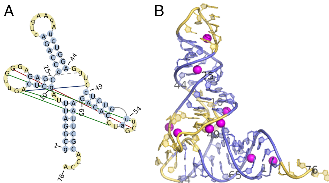
Figure 3.2: Canonical structures of tRNA and the role of tertiary contacts and metal ions in the stabilization of RNA. A. Cloverleaf Secondary structure: the paired regions are indicated in blue, the unpaired regions in yellow; the presence of tertiary contacts (remote paired nucleotides) established between different unpaired regions (yellow) from different domains of the tRNA is indicated by brown and green lines. B. L-shape 3D structure using the same color code for the paired/unpaired regions; the metal ions ( Mg^{2+} or Mn^{2+} ) are indicated by purple spheres. The 2D and 3D structures correspond to the tRNA-Phe molecule (PDB ID: 1EHZ).
