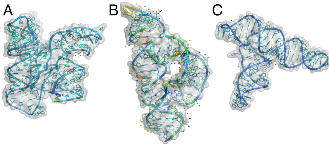
Figure 4.2: Structures of artificial and natural ribozymes with the three basic catalytic activities required for viroid replication. (A) RNA-polymerase ribozyme (PDB ID: 3IVK); the 3-D structure corresponds to a class I RNA ligase (first chemical step of RNA polymerization); a fully active RNA-polymerase ribozyme (capable of catalysing the accurate synthesis of an RNA sequence longer than itself) adopts the same 3-D fold. (B) Hammerhead ribozyme (PDB ID: 2OEU) with an RNase-like activity (self-cleaving). (C) RNA ligase ribozyme (PDB ID: 2OIU). The small coloured dots in and around the three structures indicate the presence of tightly bound metal ions and water molecules.
