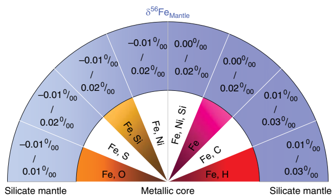
Figure 4 | Predicted shifts in the iron isotopic composition of the silicate mantle due to core formation. Schematics for \delta^{56}\text{Fe} isotope signatures in the bulk silicate Earth (primitive mantle) with regard to varying compositional models of Earth's core. The segregating metal was assumed to equilibrate with the silicate mantle at the base of the magma ocean at \sim 50 GPa and 3,500 K based on refs 45–47.
