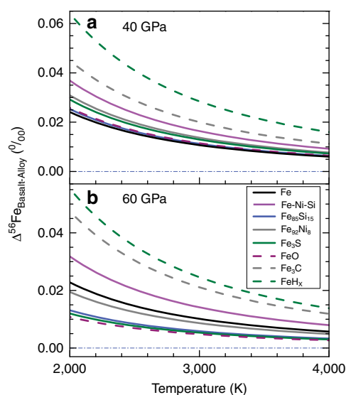
Figure 3 | Equilibrium ^{56}\text{Fe}/^{54}\text{Fe} isotope fractionation between basaltic glass and iron-rich alloys at high pressure and temperature. a . Pressure at 40 GPa. b . Pressure at 60 GPa. Black, magenta, blue, grey and olive solid lines: Fe, \text{Fe}_{86.8}\text{Ni}_{8.6}\text{Si}_{4.6} , \text{Fe}_{85}\text{Si}_{15} , \text{Fe}_{92}\text{Ni}_8 , and \text{Fe}_3\text{S} alloys, respectively, from this study. Purple, grey and olive dashed lines: \text{FeO} , \text{Fe}_3\text{C} and \text{FeH}_x , respectively, from Shahar et al. 25 \Delta^{56}\text{Fe}_{\text{Basalt-Alloy}} = \delta^{56}\text{Fe}_{\text{Basalt}} - \delta^{56}\text{Fe}_{\text{Alloy}} . Blue dash-dotted lines represent no iron isotopic fractionation between basaltic glass and Fe-rich alloys.
