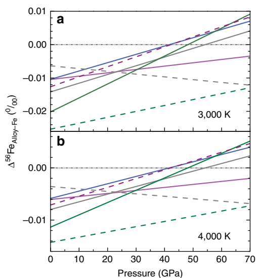
Figure 2 | Comparisons of \beta -factors of iron-rich alloys at high pressure and temperature. Difference in the ^{56}\text{Fe}/^{54}\text{Fe} \beta -factors of iron-rich alloys with respect to pure iron at 3,000 K ( a ) and 4,000 K ( b ) as a function of pressure. Magenta, blue, grey and olive solid lines: \text{Fe}_{86.8}\text{Ni}_{8.6}\text{Si}_{4.6} , \text{Fe}_{85}\text{Si}_{15} , \text{Fe}_{92}\text{Ni}_8 and \text{Fe}_3\text{S} alloys, respectively, from this study. Purple, grey and olive dashed lines: \text{FeO} , \text{Fe}_3\text{C} and \text{FeH}_x , respectively, from Shahar et al. 25 \Delta^{56}\text{Fe}_{\text{Alloy-Fe}} = \delta^{56}\text{Fe}_{\text{Alloy}} - \delta^{56}\text{Fe}_{\text{Fe}} = 1,000 \times (\ln \beta_{\text{Alloy}}^{56/54}\text{Fe} - \ln \beta_{\text{Fe}}^{56/54}\text{Fe}) . Black dash-dotted lines represent no iron isotopic fractionation between Fe-rich alloys and pure iron.
