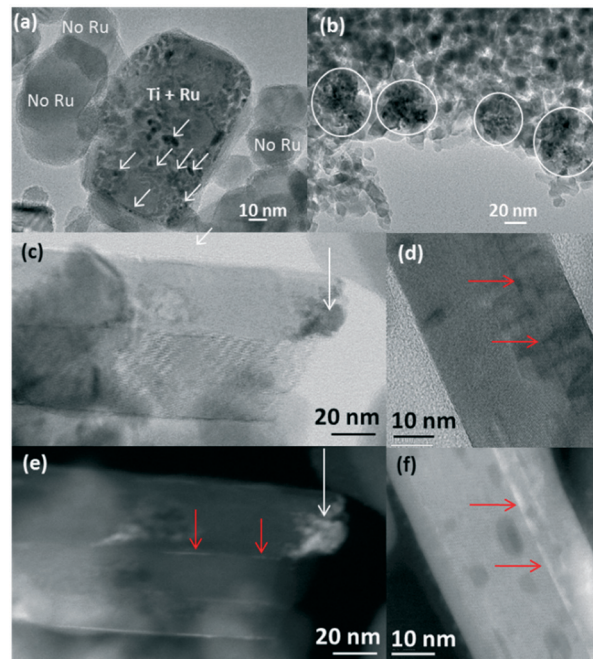
Fig. 7 TEM images of the catalysts post reduction and methanation: (a) \text{Ru/TiO}_2\text{-P25-450} post methanation showing Ru-free anatase \text{TiO}_2 and Ru-covered rutile \text{TiO}_2 particles; (b) \text{Ru/TiO}_2\text{-A-450} post methanation showing agglomerated Ru particles (indicated by white circles); bright field (c and d) and HAADF (e and f) images of \text{Ru/TiO}_2\text{-R-450} post methanation. The white arrows show the metallic Ru, and the red arrows show the trapped \text{RuO}_2 .
