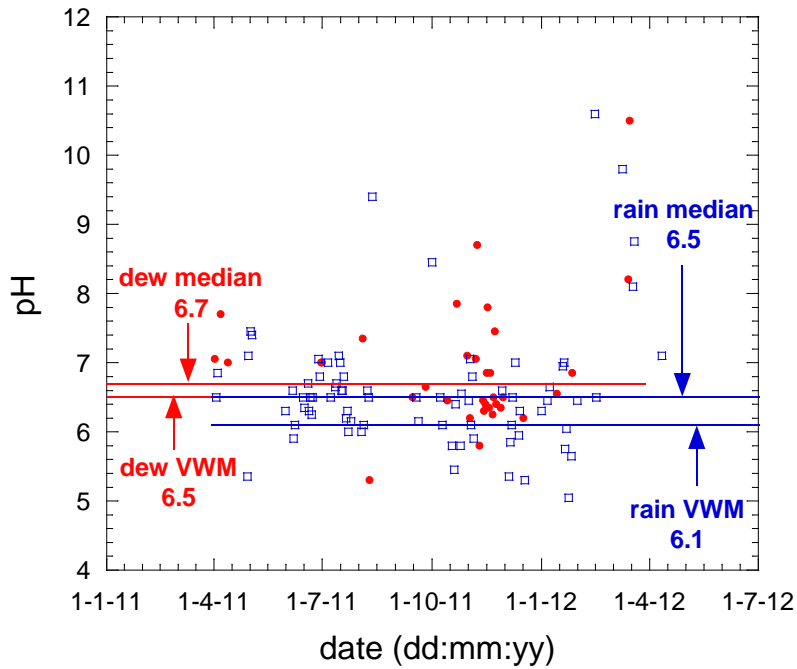
Fig. 3. Dew pH (full circles) and rain (open squares) evolution. The lines are volume weighted mean values (VWM) and median values (from Tables 2-3).
