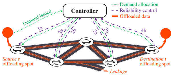
Fig. 5: Controller-to-offloading spot communication for the hop-by-hop (dashed arrows 1a-3a and 2b-4b) and end-to-end (dashed arrows 1a, 4b) retransmission strategies.
