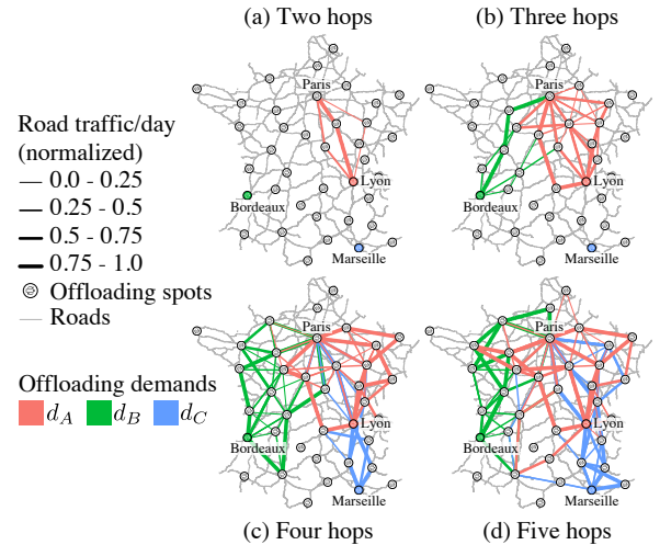
Fig. 11: Representation of the allocation of demands d_A , d_B , and d_C resulting of the strategy with controller with different values for the maximal length of the candidate logical paths.
