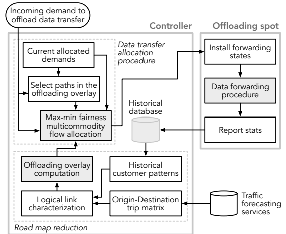
Fig. 6: Interactions between the functions of the controller and those of the offloading spots.
