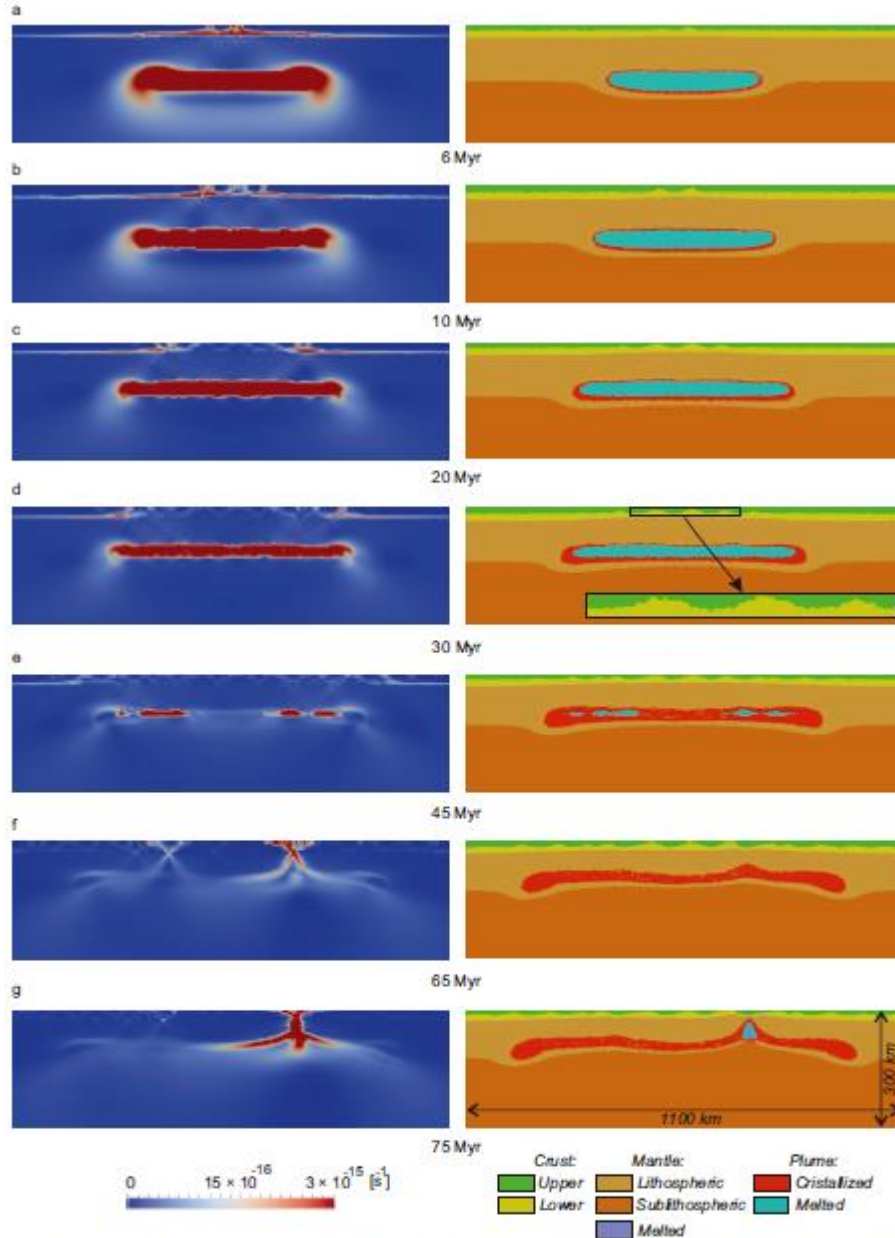
Figure 3. Reference model 1. Strain rate (left column) and compositional (right column) cross-sections: a) localized brittle deformation in the upper crust and distributed ductile strain into weak lower crust; b-d) crustal boudinage due to ductile flow in the lower crust; in-sequence migration of the brittle deformation leads to the opening of the rift basin; e) almost complete recrystallization of the plume material (note spatial position of the last melted segments); wide rift basin (~800 km) with less expressed fault boundaries; f) initiation of localized plume uplift and development of two faults zones cutting the entire lithosphere; g) continental break-up along right narrow rift (note that left rift is abandoned); decompressional melting of plume and lithospheric material due to its localized uplift underneath the spreading axis.
