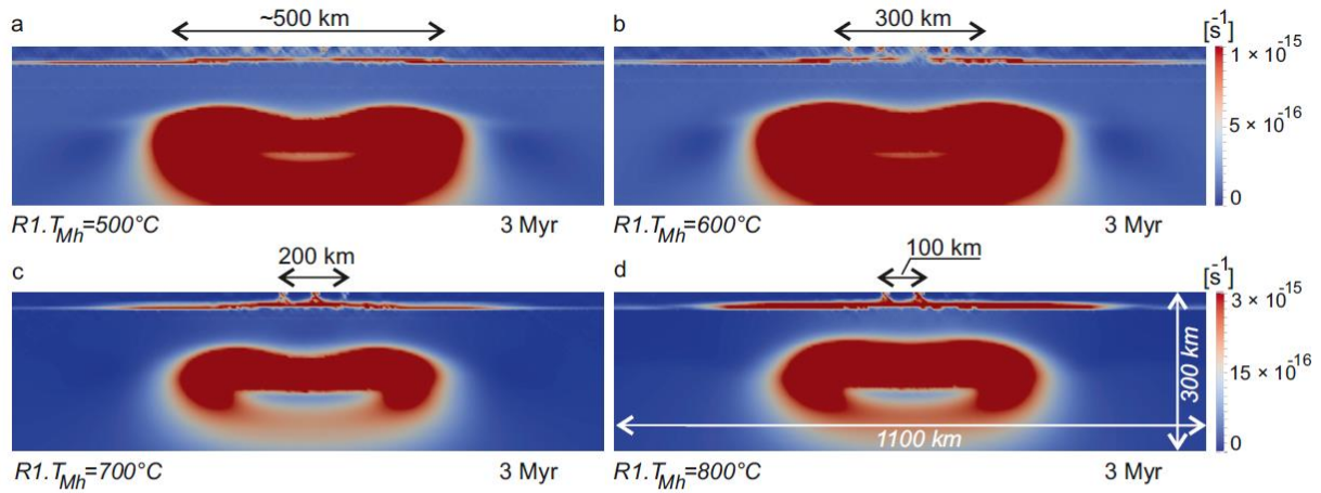
Figure 8. Strain rate cross-sections through a) model 3 (Moho temperature of 500^\circ\text{C} ); b) model 4 (Moho temperature of 600^\circ\text{C} ); c) reference model 1 (Moho temperature of 700^\circ\text{C} ) and d) model 5 (Moho temperature of 800^\circ\text{C} ) at 3 Myr.
