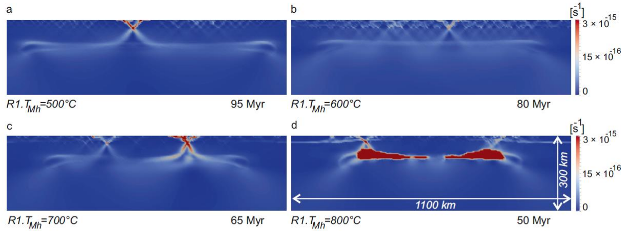
Figure 11. Strain rate cross-sections through a) model 3 (Moho temperature of 500^\circ\text{C} ); b) model 4 (Moho temperature of 600^\circ\text{C} ); c) reference model 1 (Moho temperature of 700^\circ\text{C} ) and d) model 5 (Moho temperature of 800^\circ\text{C} ) at the time of narrow rift localization.
