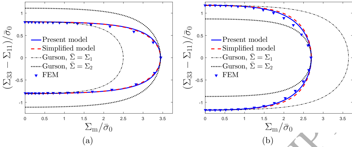
Fig. 3. Yield surfaces for isotropic pre-hardening: theoretical model given by equations (38) (Present model), simplified model given by equations (60) (Simplified model), Gurson's model (Gurson) and finite element results (FEM). (a) Case 1, (b) Case 2 (see text).
