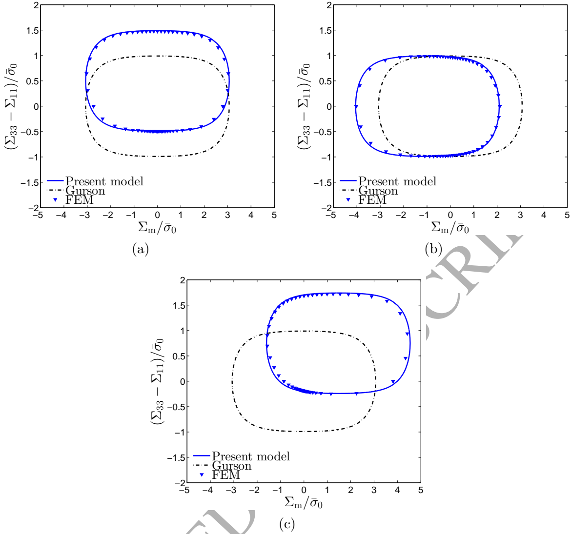
Fig. 4. Yield surfaces for kinematic pre-hardening: theoretical model given by equations (38) (Present model), Gurson's model without hardening (Gurson) and finite element results (FEM). (a) Case 1, (b) Case 2, (c) Case 3 (see text).
