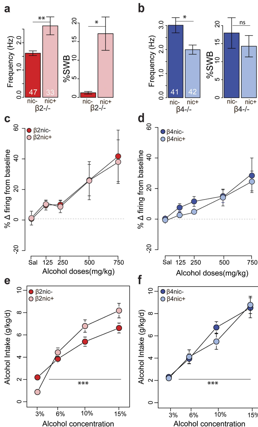
Figure 4. Alcohol-elicited responses and alcohol intake of \beta 2^{-/-} and \beta 4^{-/-} mice are not modified by chronic nicotine. (a) Barplot of the mean frequency and %SWB for \beta 2\text{nic-} (red, n = 47 ) and \beta 2\text{nic+} mice (pink, n = 33 ). ** p < 0.01 , t-test; * p < 0.05 , Wilcoxon test. (b) Barplot of the mean frequency and %SWB for \beta 4\text{nic-} (blue, n = 41 ) and \beta 4\text{nic+} mice (light blue, n = 42 ). * p < 0.05 , t-test. (c) Dose- response curves of ethanol-elicited DA cell responses for \beta 2\text{nic-} (red) and \beta 2\text{nic+} (pink). \beta 2\text{nic-} : saline: n = 15 ; 125 mg/kg: n = 5 ; 250 mg/kg: n = 10 ; 500 mg/kg: n = 11 ; 750 mg/kg: n = 8 ; \beta 2\text{nic+} : saline: n = 12 ; 125 mg/kg: n = 6 ; 250 mg/kg: n = 7 ; 500 mg/kg: n = 10 ; 750 mg/kg: n = 5 . (d) Dose- response curves of ethanol-elicited DA cell responses for \beta 4\text{nic-} (blue) and \beta 4\text{nic+} (light blue). \beta 4\text{nic-} : saline: n = 23 ; 125 mg/kg: n = 9 ; 250 mg/kg: n = 10 ; 500 mg/kg: n = 14 ; 750 mg/kg: n = 7 ; \beta 4\text{nic+} : saline: n = 15 ; 125 mg/kg: n = 7 ; 250 mg/kg: n = 10 ; 500 mg/kg: n = 8 ; 750 mg/kg: n = 6 . (e) Mean \pm SEM of ethanol consumption (gr/kg) in \beta 2\text{nic-} (red, n = 9 ) and \beta 2\text{nic+} (pink, n = 8 ) mice during the two bottle choice procedure. (f) Mean \pm SEM of ethanol consumption (gr/kg) in \beta 4\text{nic-} (blue, n = 6 ) and \beta 4\text{nic+} (light blue, n = 6 ) mice during the two bottle choice procedure.
