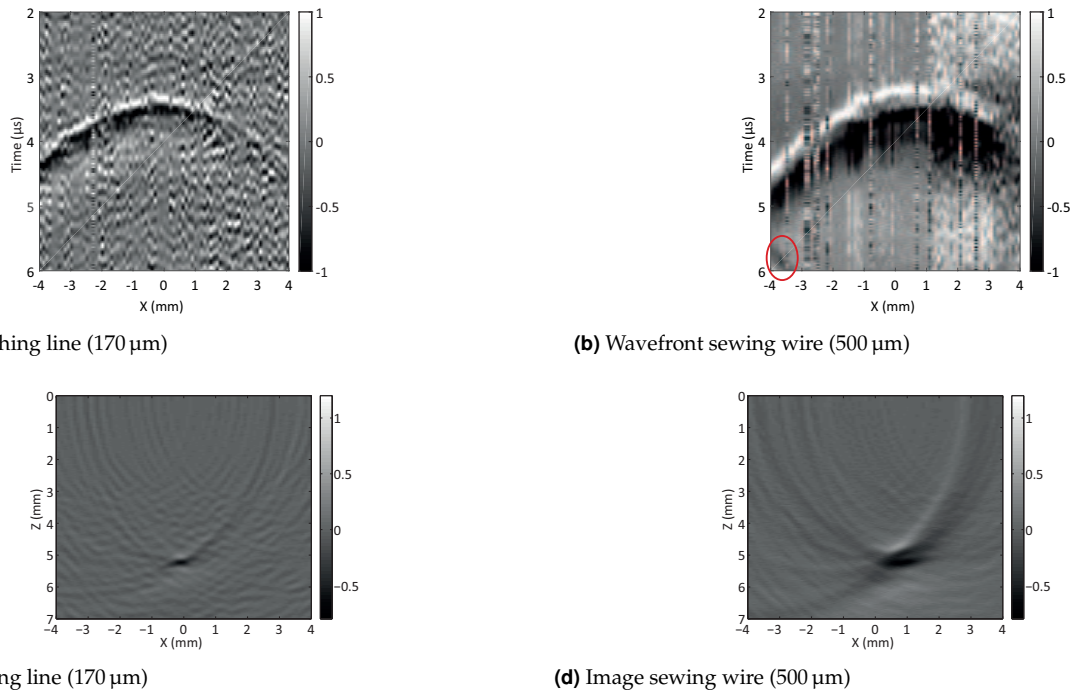
Fig. 6. Time signals at different positions for the fishing line(a) and for the sewing wire(b) (The red circle corresponds to parasitic reflection on one of the edges of the gel.). Image after beamforming for the fishing line(c) and for the sewing wire(d).
