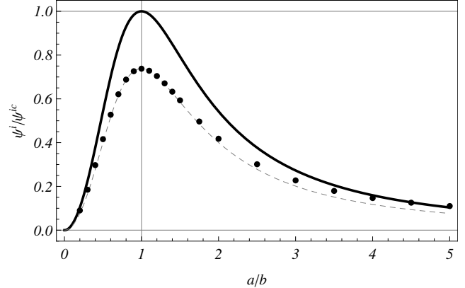
Fig. 4 The ratio \psi^i/\psi^{ic} for isotropic material as function of the planform aspect ratio a/b : exact solution for ellipses (black), FE solution (points) and the approximation (16) (dashed) for rectangular planform.
