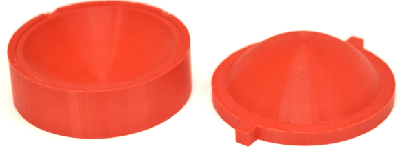
Fig. 11 Mold with radius of curvature 5.5 cm used to build the tristable shell in Figure 10.
