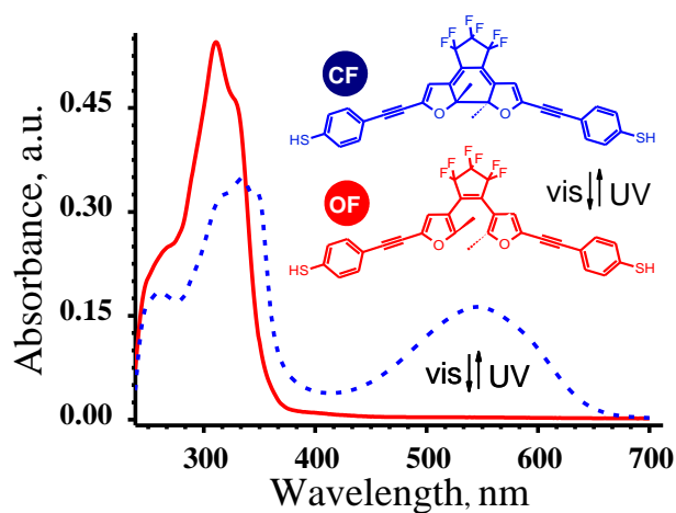
Figure 1. Temporal evolution of absorption spectra of YnPhT molecules in ethanol showing the reversible transition between OF \leftrightarrow CF upon irradiation with either visible light or UV irradiation with \lambda = 254 nm. Inset show structural changes in hexafluorocyclopentene photochromic core of YnPhT during ultraviolet/visible (UV/vis) light irradiation.
