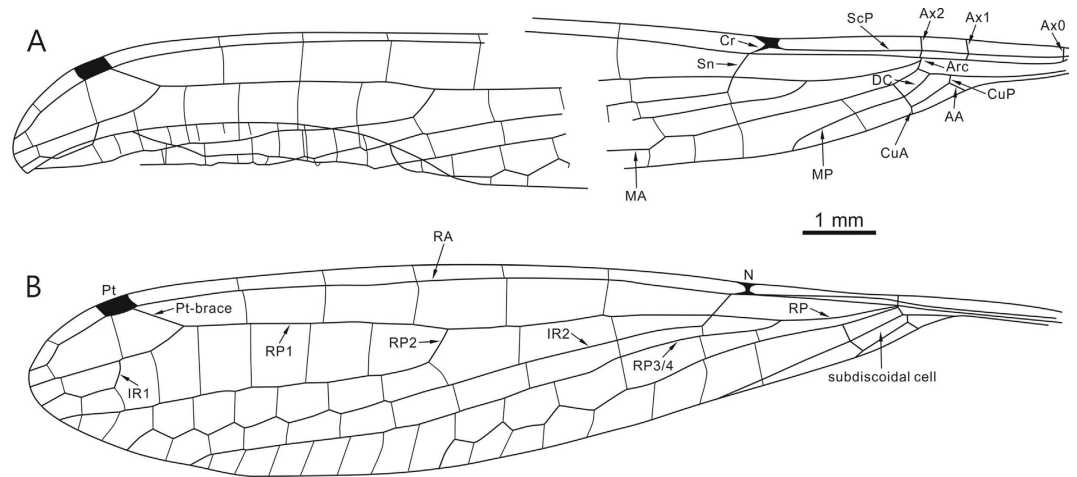
Figure 4. Yijenplatycnemis huangi gen. et sp. nov. Paratype (BA16200); line drawing showing venation of left forewing (A) and hindwing (B) (drawn by DZ). Abbreviations: AA, anterior anal; Arc, arculus; Ax, primary antenodal crossvein; Cr, nodal crossvein; CuA, cubitus anterior; CuP, cubitus posterior; DC, discoidal cell; IR, intercalary radial vein; MA, median anterior; MP, median posterior; N, nodus; Pt, pterostigma; RA, radius anterior; RP, radius posterior; ScP, subcosta posterior; Sn, subnodal crossvein.
