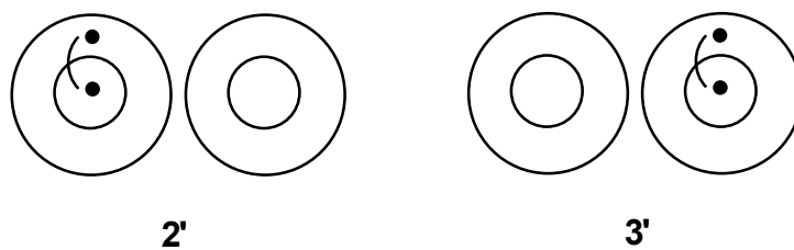
Figure 2. Schematic representation of the active orbital splitting in the main ionic structures at the SL-BOVB level. The dots represent the two electrons of the 4s-type pair, and the curve connection the dots indicate a singlet coupling between the two electrons in the two split orbitals 2a and 2b (resp. 3a and 3b) in structure 2' (resp. 3' ).
