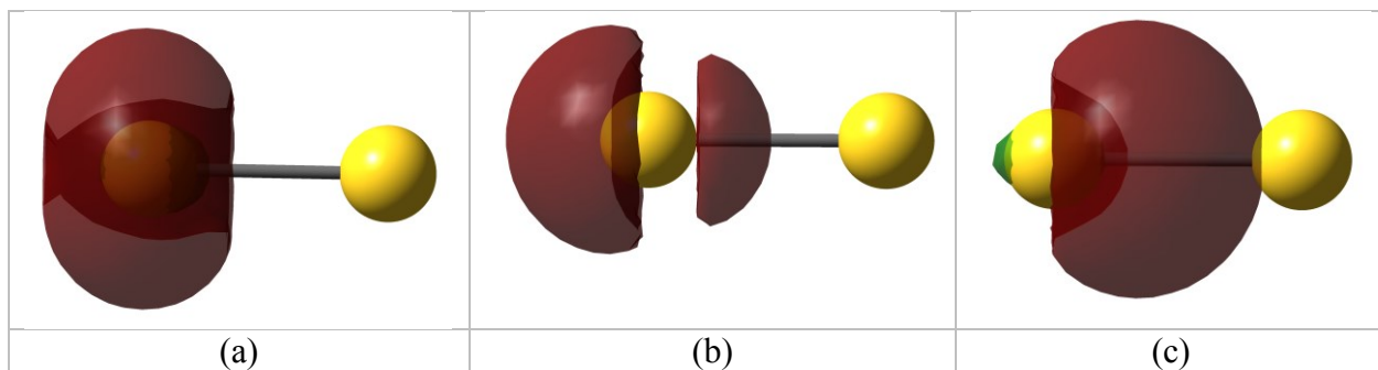
Figure 3. Computed 4s-type VB orbitals of \text{Au}_2 at the SL-BOVB level, (a): in the covalent structure 1 , and (b) and (c): the “split” pairs of orbitals in the ionic structure 2' (see Figure 2 for a schematic representation of this VB structure).
