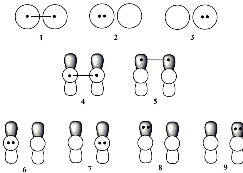
Figure 1. VB basis of structures for the 2c/2e bond of the coinage metal dimers.
