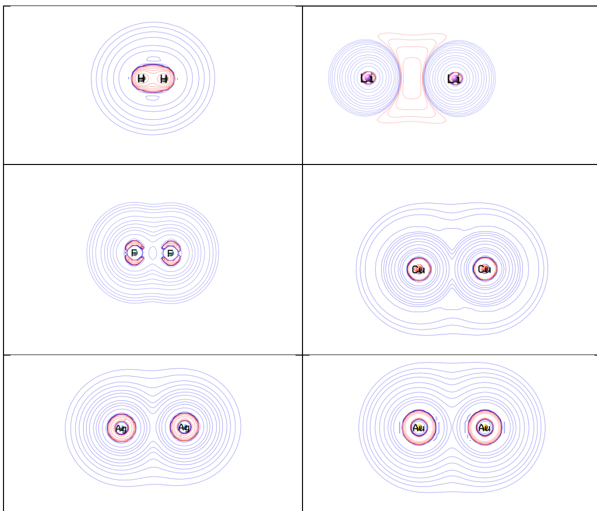
Figure 4. Distribution of \nabla^2\rho in the xz -plane (atoms lay along the z -axis). Blue lines indicate areas of charge depletion (positive values of \nabla^2\rho ) and red lines indicate areas of charge concentration (negative values of \nabla^2\rho ). The H_2 and Li_2 molecules (top left and right drawings respectively) provides example of covalent bonding, while F_2 (middle left) provides an example of complete Charge Shift Bond. The coinage metal dimers correspond to middle right ( Cu_2 ), bottom left ( Ag_2 ) and bottom right ( Au_2 ) figures.
