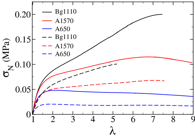
Fig. 3. Nominal stress versus elongation in tensile test for an elongation rate \lambda_z = 0.07 \text{ s}^{-1} (solid lines) and \lambda_z = 0.007 \text{ s}^{-1} (dashed lines).
