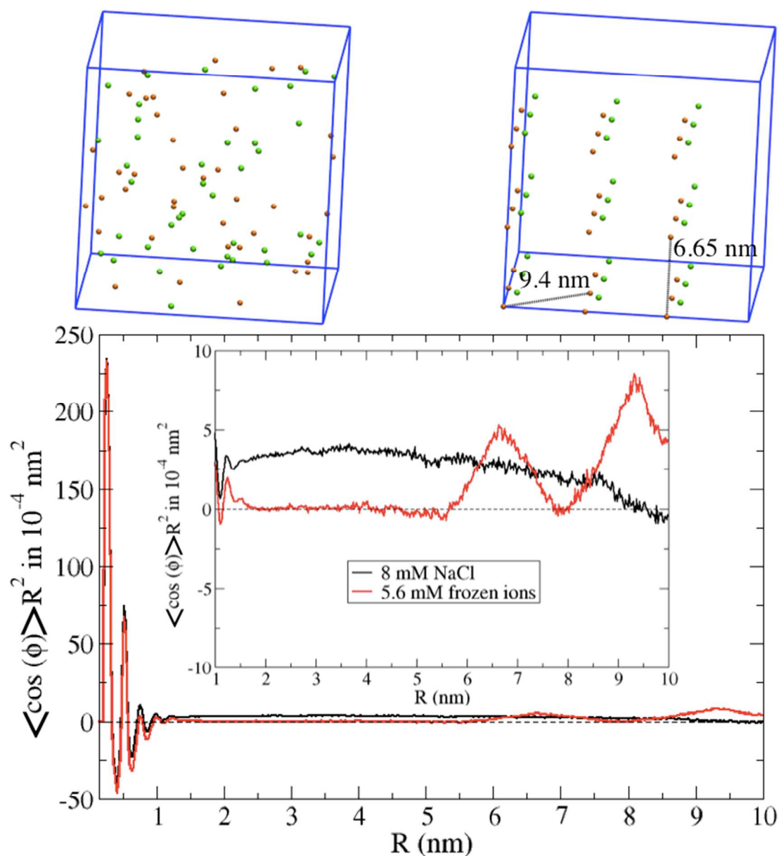
Figure 1. Top: Snapshots of ionic arrangements in an unconstrained 8 mM NaCl solution (left) and in a 5.6 mM NaCl solution with a fixed regular arrangement of ions (right). Bottom: The corresponding distance-weighted water-water orientational correlation functions (black and red lines). The inset zooms in the correlation for distances larger than 1 nm.
