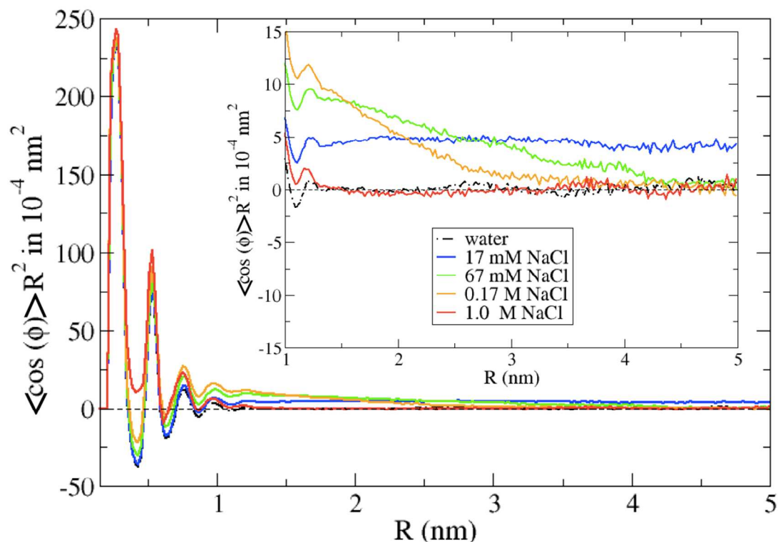
Figure 4. Concentration dependence of distance weighted water-water orientational correlation in a \sim 10 nm simulation cell, comparison of neat water (black dashed-dotted line) and solutions with different NaCl concentration (color solid lines). The inset zooms in the correlation for distances larger than 1 nm.
