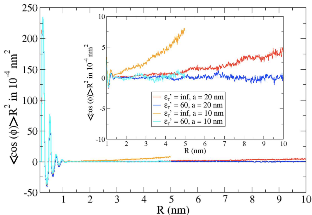
Figure 3. Distance-weighted water-water orientational correlation functions in neat water. Comparison of two types of Ewald boundary conditions - a tin foil \epsilon_r' = \infty (red) vs. \epsilon_r' = 60 (blue) for two sizes of the unit cell of approximately 10 and 20 nm. The inset zooms in the correlation functions for distances larger than 1 nm.
