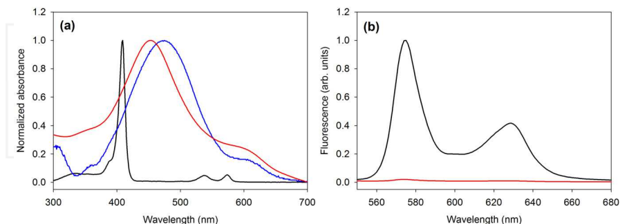
Fig. 10. (a) Normalized UV-visible absorption spectra of ZnOEP in DMF ( \blacksquare ), of an ITO electrode modified with the polymer obtained from ZnOEP and bpy after 25 iterative scans ( \blacksquare ) and of this same polymer in solution in DMF ( \blacktriangle ). (b) Luminescence spectra of ZnOEP ( \blacksquare ) and of the polymer obtained from ZnOEP and bpy ( \blacktriangle ) in DMF. \lambda_{\text{exc}} = 420 \text{ nm} .
