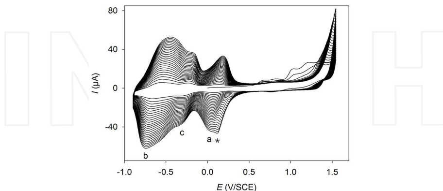
Fig. 8. Cyclic voltammograms recorded during the iterative scans between -0.90 and +1.60 V/SCE of \text{ZnOEP} ( 0.25 mM) in the presence of \text{bpy} ( 0.25 mM) in 1,2\text{-C}_2\text{H}_4\text{Cl}_2 and 0.1 M \text{NEt}_4\text{PF}_6 . Working electrode: ITO; S = 1 cm 2 ; v = 0.2 V s -1 .
