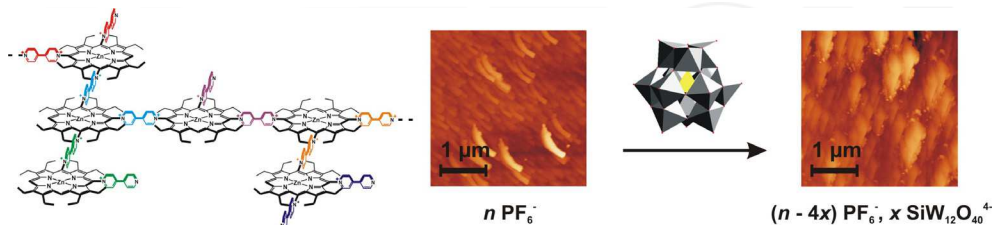
Fig. 22. Atomic force micrographs of an ITO electrode coated with the polymer obtained from 5,10-ZnOEP(bpy) _2^{2+} after plunging for 10 hours in water (left) and in a solution of \text{SiW}_{12}\text{O}_{40}^{4-} (1 mM) (right).
