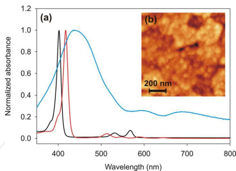
Fig. 15. (a) Normalized UV-visible absorption spectra of ZnOEP in 1,2- C_2H_4Cl_2 (—), of 5,15- H_2Py_2Ph_2P in 1,2- C_2H_4Cl_2 (—) and of an ITO electrode modified with the copolymer obtained from ZnOEP and 5,15- H_2Py_2Ph_2P after 25 iterative scans (—). (b) Atomic force micrograph of the same copolymer after washing with water.
