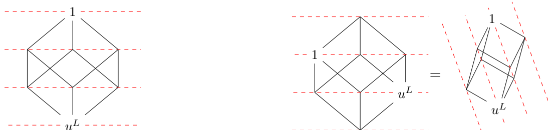
(a) Hasse diagram for an \mathfrak{su}(3) spin chain's Q-functions: the Q-functions of figure 5 are not written explicitly, only the conditions Q_\emptyset = 1 and Q_\emptyset^{[s_0]} = u^L are made manifest (the shift [s_0] is omitted).
