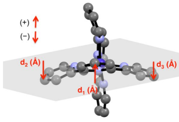
Figure 5. (a) Deviation from orthogonality descriptors: acute angle \alpha and obtuse angle \beta (averaged N_{\text{dist}}\text{-Co-}N_{\text{dist}} angles); (b) Deviation from planarity descriptors d_1 , d_2 , d_3 (the three N-atoms of the ligand define a plane). Arbitrarily, the central ring is always defined above the plane. Deviations above or below the plane are denoted with + and -, respectively.
