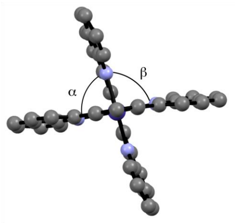
Figure 5. (a) Deviation from orthogonality descriptors: acute angle \alpha and obtuse angle \beta (averaged N_{\text{dist}}\text{-Co-}N_{\text{dist}} angles); (b) Deviation from planarity descriptors d_1 , d_2 , d_3 (the three N-atoms of the ligand define a plane). Arbitrarily, the central ring is always defined above the plane. Deviations above or below the plane are denoted with + and -, respectively.
