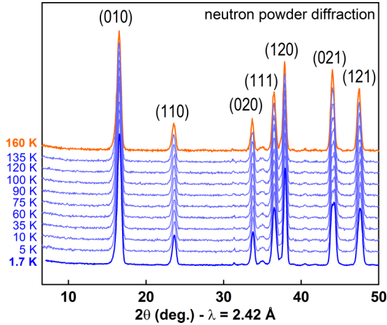
FIG. 9. Evolution of the neutron powder diffraction patterns ( \lambda = 2.42 \text{ \AA} ) of \text{Li}_2\text{Cu}_2\text{O}(\text{SO}_4)_2 while cooling the sample from 160 K (above the transition) down to 1.7 K. (hkl) indexes refer to the tetragonal cell. Note the absence of any peak arising at low angle, nor diffuse background of magnetic origin.
