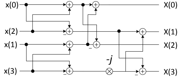
(c) Radix-4
