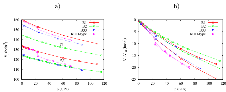
Fig. 6 a) Evolution of Bader volumes V_i upon compression in the B1, B2 B33 and KOH-type phases. b) \Delta V_i = V_{i,p} - V_{i,0} for each of the previous phases. Ag in squares and Cl in crosses.
