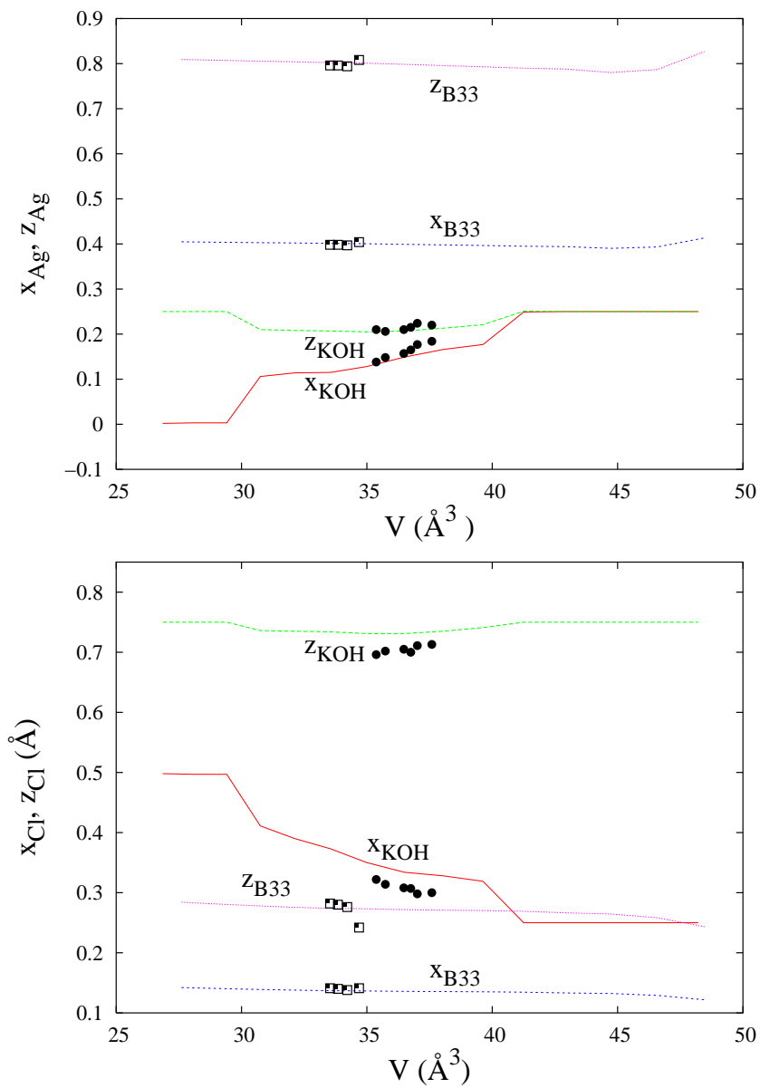
Fig. 3 Variation of Ag position with volume according to our GGA calculations (solid lines) and available experimental data (symbols).[15] Black dots and white squares stand, respectively, for the KOH-type and B33 structures. All data referred to the P2_1/m unit cell.
