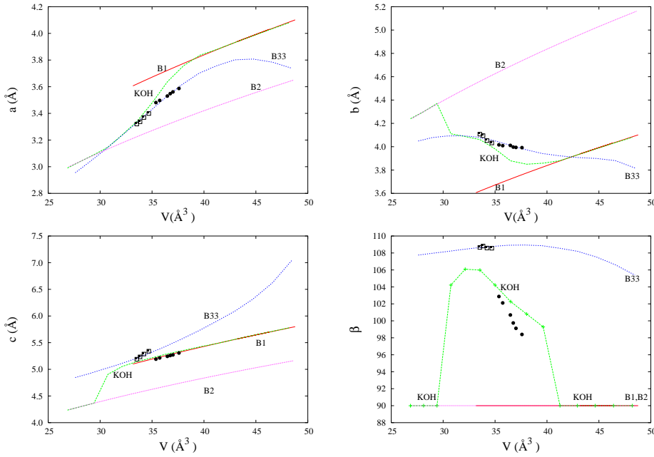
Fig. 2 Variation of the unit cell parameters with volumen according to our GGA calculations (solid lines) and available experimental data (symbols).[15] Black dots and white squares stand, respectively, for the KOH-type and B33 structures. All data referred to the P2_1/m unit cell.
