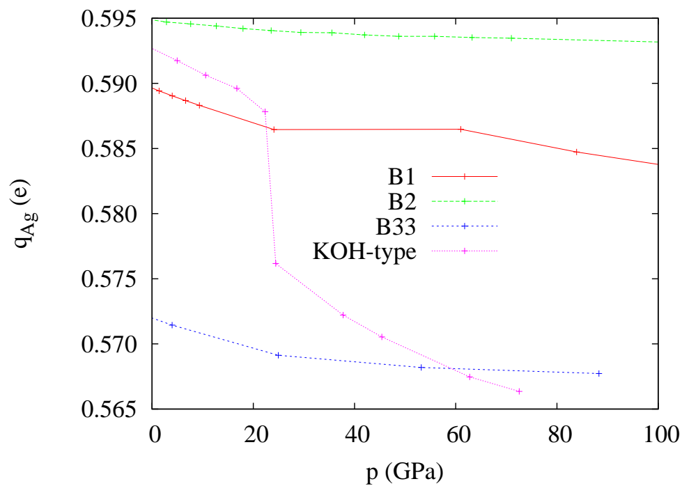
Fig. 5 Evolution of Bader charges upon compression in the B1, B2, B33 and KOH-type phases.
