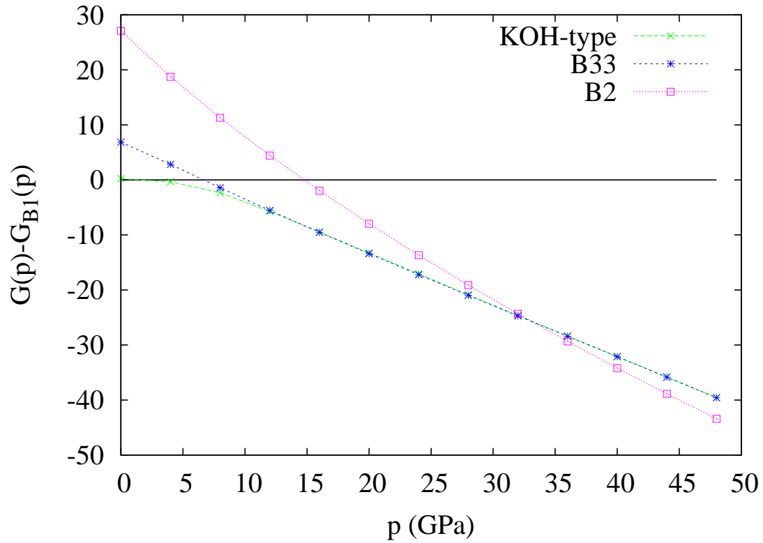
Fig. 4 Gibbs energy relative to B1 gibbs energy vs. pressure.
