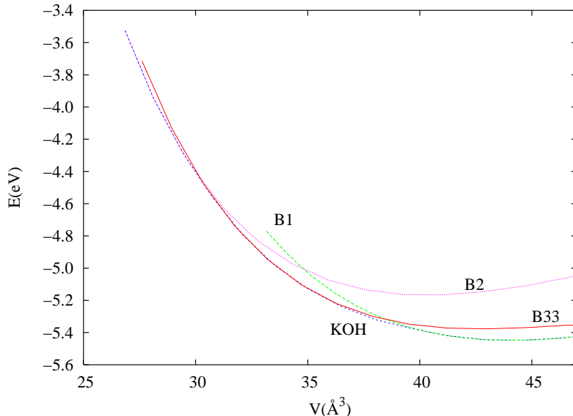
Fig. 1 Energy-volume curves for the B1, KOH-type, B33 and B2 polymorphs of AgCl according to our GGA calculations. It can be seen how the energy of the KOH-type structure coincides with that of the cubic and orthorhombic lattices at different volume ranges. In the case of B1 and B2 phases, this coincidence is complete as they constitute different representations of the same structure. However, this is not the case for B33 (TII-type), which presents a degeneration with a distorted anti-TII structure.
