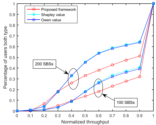
FIGURE 7. Throughput Cumulative Distribution Function for users of both types: Comparison of the proposed framework with other coalitional games.
