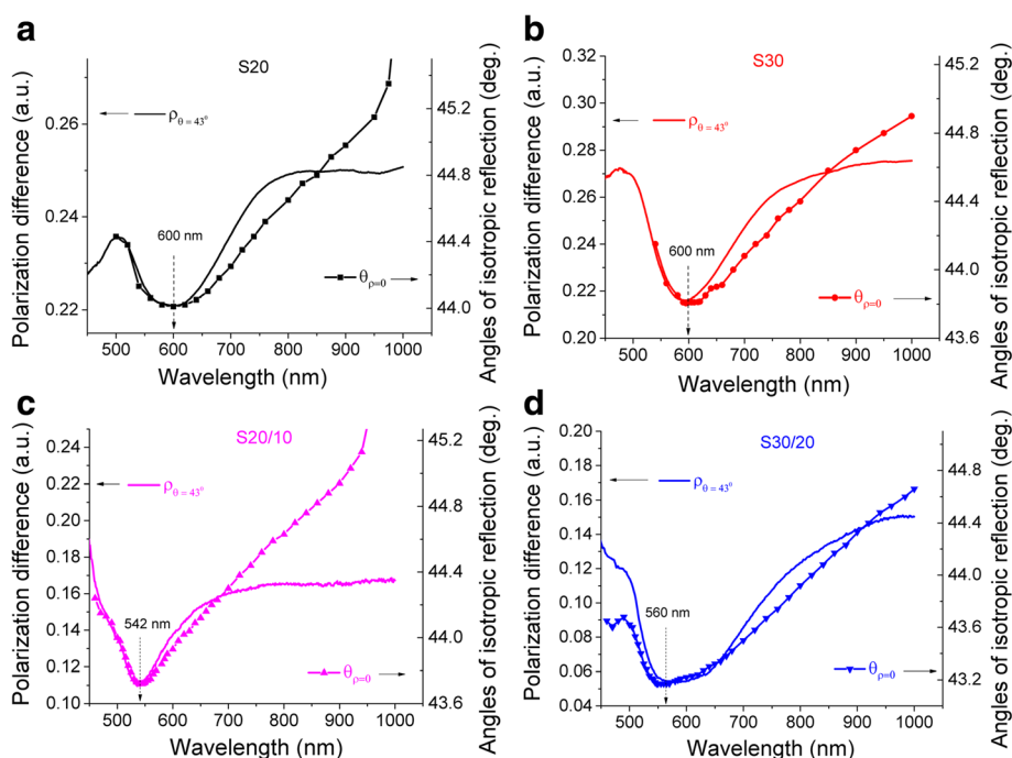
Fig. 7 Spectral dependencies of the angles of isotropic reflection \theta_{\rho=0}(\lambda) in comparison with the spectral dependencies of the polarization difference \rho(\lambda) at incident angle of light \theta = 43^\circ for samples S20 (a), S30 (b) of single AuNP, and S20/10 (c), S30/20 (d) of AuNP dimers
