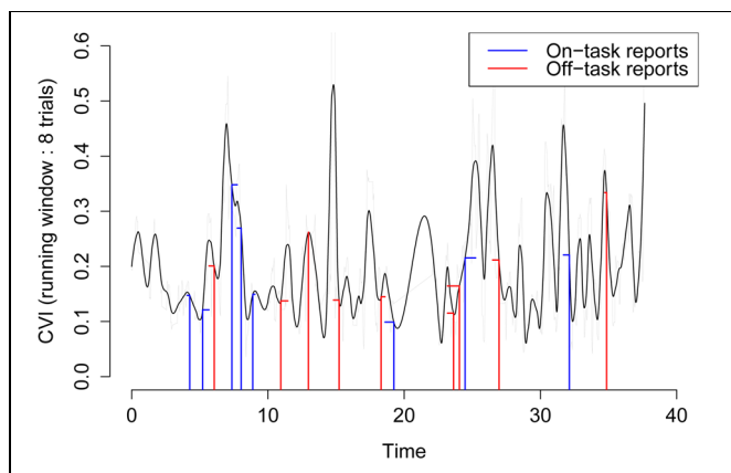
FIGURE 2 | Distribution of the Continuous Variability Index (CVI) across the experimental session of an arbitrary participant (time in minutes).
