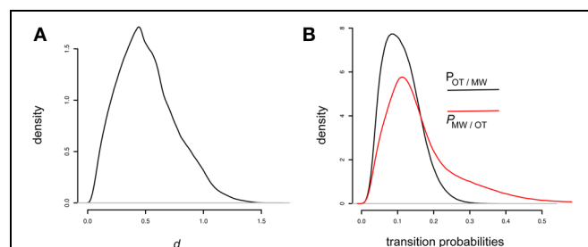
FIGURE 5 | (A) Overall posterior distribution of the parameter d in the exponential model, pooled across all 47 participants (60000 samples per participant). Note that the prior was uniform over [0, 2] . (B) Overall posterior distribution of the two transition probabilities in the exponential model. The prior was uniform over [0, 1] (60000 samples per participant).
