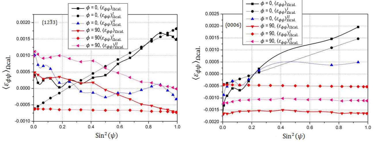
Fig. 9: Calculated elastic strains \langle \varepsilon_{\phi\psi} \rangle_{\Omega_{cal}} as a function of \sin^2 \psi for Point 4 (elastic reloading after elastoplastic loading and unloading) on the tensile curve; the macroscopic elastic strain depends again on both 1 st and 2 nd order stress tensors; \langle \varepsilon_{\phi\psi} \rangle_{\Omega_{cal}} = \langle \varepsilon_{\phi\psi} \rangle_{\Omega_{cal}}^I + \langle \varepsilon_{\phi\psi} \rangle_{\Omega_{cal}}^{II} .
