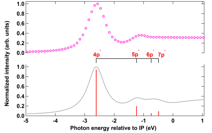
FIG. 3. Experimental (top curve) and reconstructed (bottom curve) PEY. The bars under the reconstructed PEY indicate the intensities of the 1s - mp absorption transitions ( 4 \leq m \leq 7 ), extracted from the fitting procedure; the solid line is the sum of the discrete contributions and the continuum contribution fitted with an arctangent function.
