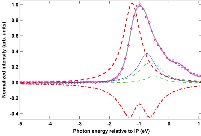
FIG. 2. Cross section of the 2p^{-2}6p^{+} final state plotted as a function of the photon energy relative to the ionization potential. The circles are the experimental points, the thick solid gray line is the fitting result. The thin solid blue, thick dashed red, and thin dashed green lines show the contributions of the spectator decay, the decay accompanied by a shake-up process from the 5p orbital, and the decay involving a shake-down process from the 7p orbital, respectively. The interference cross terms between the 1s^{-1}6p' and 1s^{-1}5p' electronic states and between the 1s^{-1}6p' and 1s^{-1}7p' electronic states are shown with thick dash-dotted red and thin dash-dotted green lines, respectively.
