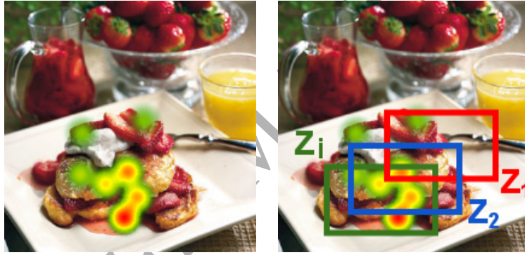
Figure 2: The rationale of the definition of gaze loss. When the color of heatmap is closer to red, the density of gaze is higher. The region contains the maximum density of gaze is shown as z_i (shown as the green rectangle). The gaze loss of z_i is thus defined as 0. The red region z_1 contains a smaller density of gaze with respect to the blue region z_2 , leading to a larger gaze loss.
