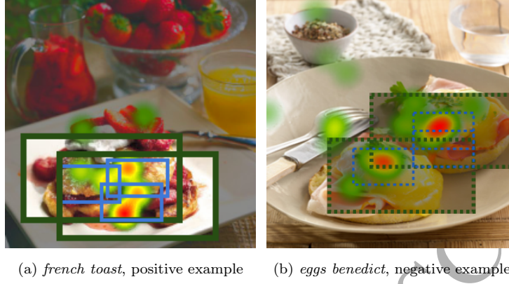
Figure 3: Illustration of top k G \pm LSVM model. Human gaze density is represented by the heat map. In our models, positive example emphasize the latent regions with high gaze density (inside the solid boxes), while negative example emphasizes the regions with low gaze density (outside the dashed boxes). Different colors of regions indicate different scales. For one scale, our model takes multiple highest scored regions as the relevant regions. (Best viewed in color)
