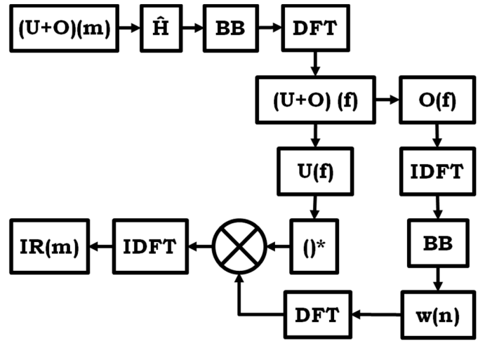
Figure III: DFT algorithm
