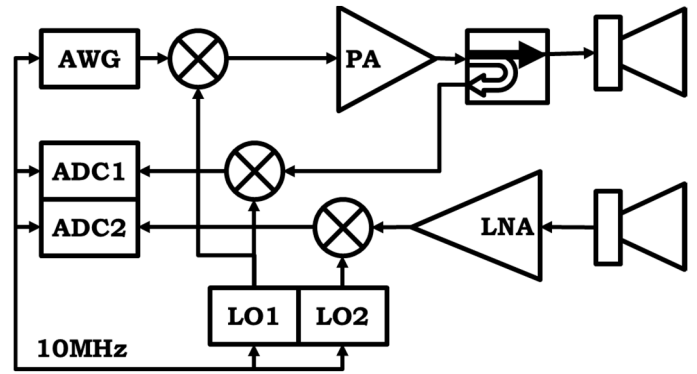
Figure I: synopsis of parallel architecture
