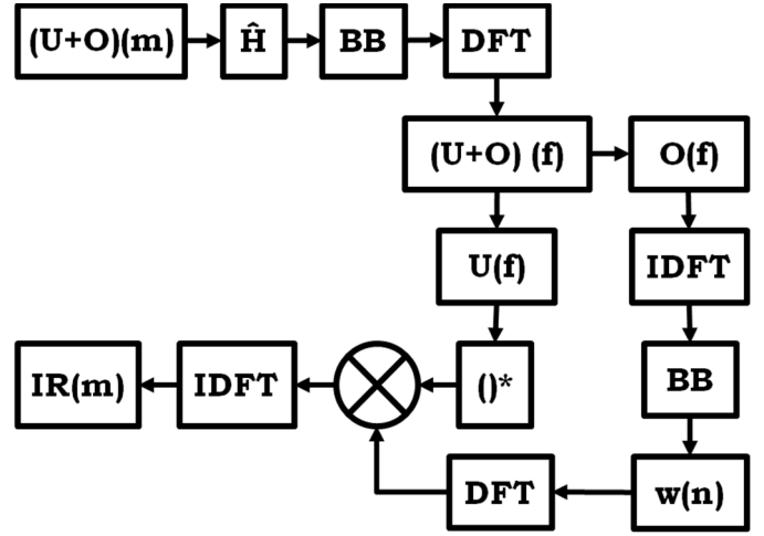
Figure III: DFT algorithm
