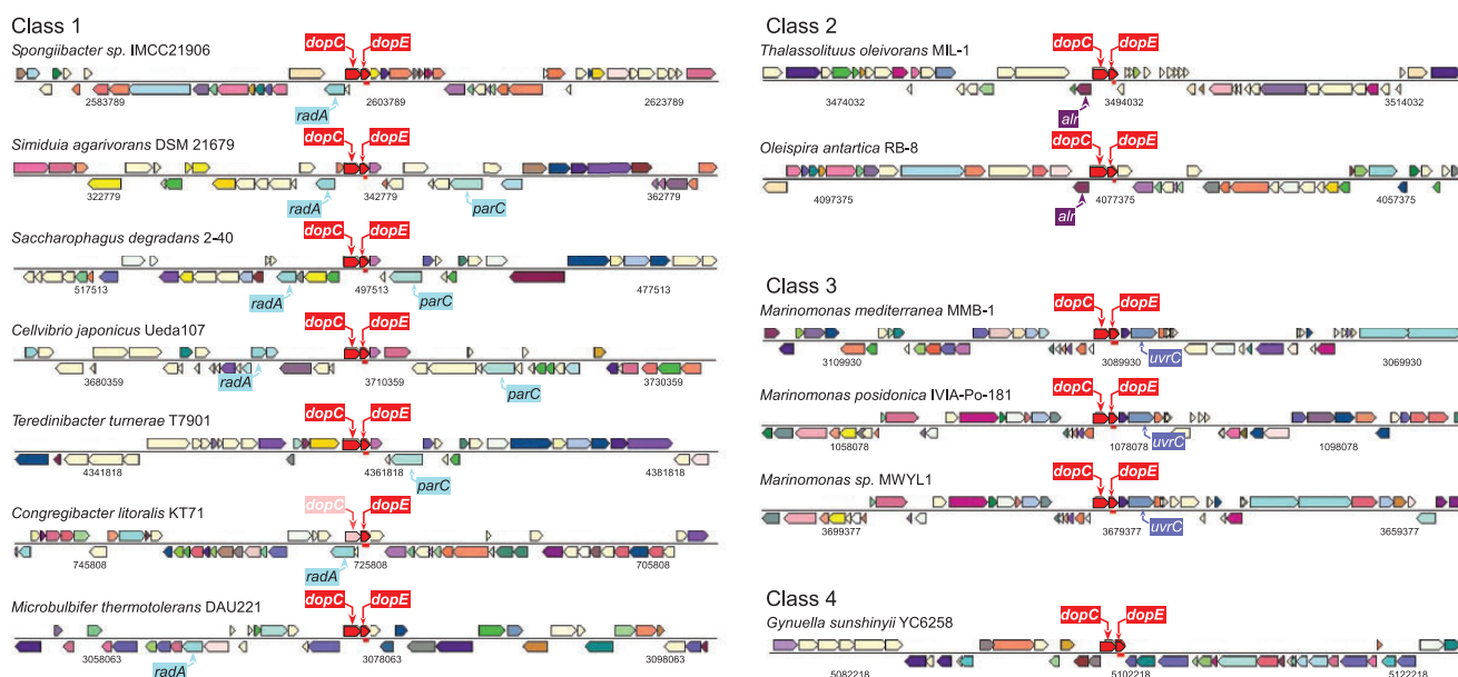
FIG. 2. — dopCE is distributed in 4 genomic context classes. The dopE gene of Cellvibrio japonicus was retrieved in the integrated microbial genome (IMG) interface at the JGI, with its locus tag (CJA_3124), and its homologs in the 12 complete genomes of Cellvibrionales and Oceanospirillales were then added in the gene list with the built-in Blast function. The “show neighborhood” tool was then used to display all 13 genetic contexts. The dopE gene and its neighboring dopC are shown in red. The position of the putative dopC gene in Congregibacter littoralis KT71 is shown in light pink as a careful inspection of the genome of this bacteria revealed the presence of a 253 residues long orf containing the characteristics of other O-like proteins, apparently missed during the annotation of this genome. In the display, genes receive a color when they belong to an identified Cluster of Orthologous Gene (COG). The result was reordered, to regroup similar contexts. Some genes typical of each class are highlighted.
