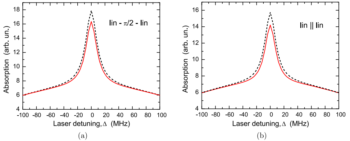
Figure 14. Illustration of the influence of cell length on the resonances in different polarization configurations: (a) perpendicular polarizations, (b) parallel polarizations. Solid red lines are obtained for a cell length L = 2 cm. Dashed black lines are obtained for L = 5 cm. Other parameters are: \Delta_R = 0 , \beta = 1 , \phi_{12} = 0 . One can see that the HFS-CPT effect makes the central absorption peak sensitive to the light-field polarizations in the cases of short- or medium-length cells ( L \lesssim 2 cm for cesium, compare amplitudes of the red-line resonances in parts (a) and (b)). At the same time, this sensitivity is absent for long cells, i.e. it is averaged along the length of a vapor cell. However, it should be emphasized that the total influence of the HFS-CPT effect on the creation of the central peak is not averaged along the cell, and the central peak caused by this effect can be observed even in the case of a long cell (see also figure 15).
