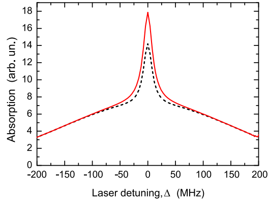
Figure 13. Absorption of the cell as a function of the one-photon detuning. The red solid curve is obtained for perpendicular polarizations ( \phi = \pi/2 ), while the black dashed curve is obtained for parallel polarizations ( \phi = 0 ). Other parameters are: \Delta_R = 0 , \beta = 1 , L = 2 cm, \phi_{12} = 0 . The peak at the center can be observed due to the HFS-CPT effect.
