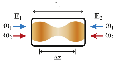
Figure 12. Picture to demonstrate inhomogeneity of light fluorescence in a vapor cell due to the HFS-CPT effect, which is sensitive to the spatial phases of the light waves.
