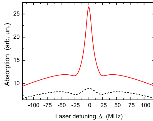
Figure 22. Study of the influence of the openness of the energy-level system on the strength of the optical pumping effect that produces the absorption spike: \beta = 1 is for a closed system (red solid line) and \beta = 0.5 is for an open system (black dashed line).
