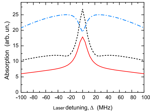
Figure 17. Absorption as a function of the one-photon detuning in the dual-frequency case with a Raman detuning \Delta_R = 0 (red solid curve), \Delta_R = 2 \Gamma (blue dash-dotted curve) or \Delta_R = 20 \Gamma (dashed black curve). Other parameters are: \phi = \pi/2 , \beta = 1 , L = 2 cm.
