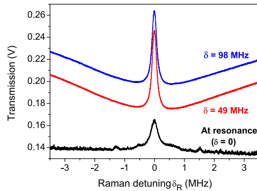
Figure 7. Coherent population trapping (CPT) spectroscopy in the reversed dip for several values of the optical detuning ( \delta = 0, 49 and 98 MHz). The static magnetic field is null. Crossed polarizations are used. The laser power is 187 \mu\text{W} . For the black curve ( \delta = 0 ), the central CPT peak can be fitted by a Lorentzian function with an FWHM of 382 kHz.
