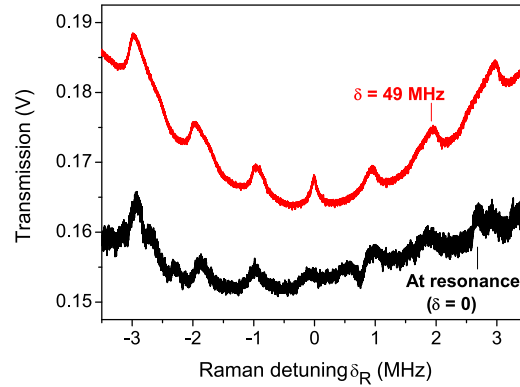
Figure 8. CPT spectroscopy in the reversed dip for two values of the optical detuning ( \delta = 0 and 49 MHz) with application of a static magnetic field ( B \sim 1.4 G). Crossed polarizations are used.
