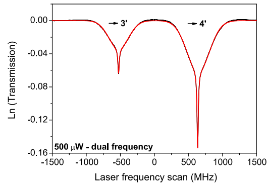
Figure 4. Doppler-free spectrum: dual-frequency laser field (a single-modulated DFB laser source), perpendicular case, B = 0 . The total laser power is 500 \mu\text{W} . Curves are fitted by the sum of Gaussian Doppler-broadened profiles and narrow Doppler-free Lorentzian dips.
