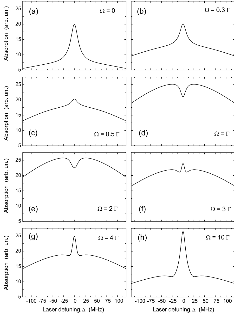
Figure 20. Influence of a longitudinal static magnetic field (i.e. the Larmor frequency \Omega \neq 0 ) on the creation of the central peak, when the Zeeman CPT effect is considered. Parameters are: \beta = 1 , \phi = \pi/2 , crossed polarizations. The central peak disappears as the Zeeman CPT states are destroyed by the magnetic field, but then it comes back due to the optical pumping effect (see section 3.3).
