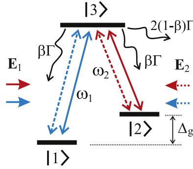
Figure 10. \Lambda -scheme of atomic energy levels. Solid vertical arrows denote transitions induced by the light-wave components with vectors \mathbf{k}_{1,2} , while dashed vertical arrows are attributed to the waves with -\mathbf{k}_{1,2} . Wavy black arrows denote spontaneous decay processes.
