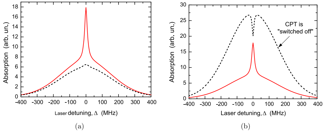
Figure 16. (a) Influence of the openness of the atomic transition on the effect of the high-contrast spike: \beta = 1 is shown by the red solid line (closed system of energy levels) and \beta = 0.5 corresponds to the black dashed line (open transition). Other parameters are: \phi = \pi/2 , \phi = 0 , \Delta_R = 0 , L = 2 cm. (b) Resonance curves obtained in the same conditions as those depicted for the red solid line of figure 13, but with the presence (red solid) or absence (black dashed) of the hyperfine CPT phenomenon.
