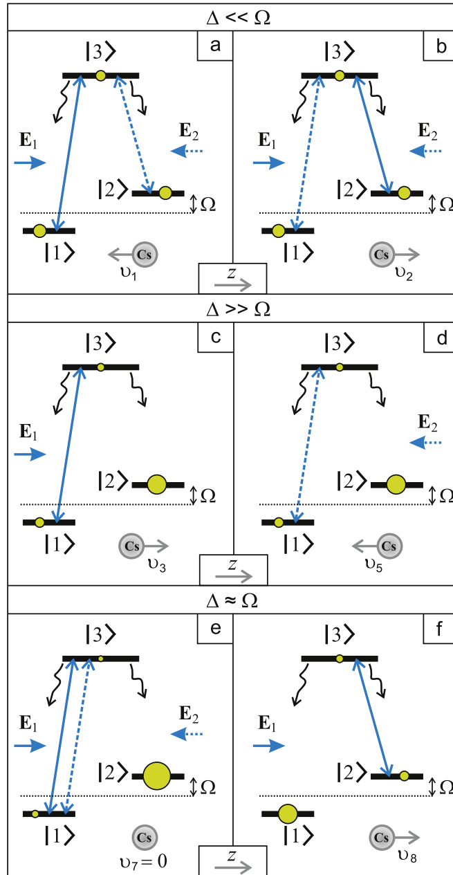
Figure 21. The three-level \Lambda -schemes show the peculiarities of population redistributions over atomic energy levels under the resonant light field in the atomic moving frame. These sketches, here for a monochromatic field, help one to understand another physical reason for observation of the central absorption peak. The branching ratio is assumed to be equal to unity ( \beta = 1 ). Light-induced transitions denoted by solid lines correspond to E_1 while dashed lines correspond to the counter-propagating E_2 wave.
