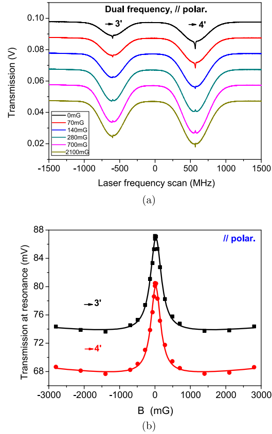
Figure 6. (a) Doppler-free spectra in the dual-frequency regime with parallel linear polarizations for several values of the static magnetic field. For clarity of the figure, offsets of -0.01 V, -0.02 V, -0.03 V, -0.04 V and -0.05 V were added to the data for the cases of B = 70, 140, 280, 700 and 2100 mG respectively. (b) From data shown in (a), the transmission peak value of the Doppler-free Lorentzian dip versus the static magnetic field (for transitions to 3' or 4' excited states). The total laser power is 187 \mu\text{W} . Experimental data are fitted by a sum of two Lorentzian functions with opposite signs.
