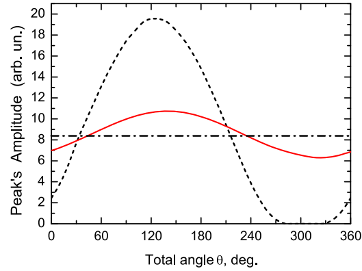
Figure 15. Influence of the total phase shift \theta = 2\phi + \phi_{12} on the amplitude of the central absorption peak for different cell lengths: L = 2 cm (solid red line) and L = 0.5 cm (dashed black line). The peak's amplitude tends to oscillate very close to the average level depicted by the dash-dotted horizontal line when the cell length is being increased. The zero gap between \theta \approx 280^\circ and 330^\circ means that there is no peak (i.e. the regular dip in the absorption is observed). The Raman detuning is assumed to be zero ( \Delta_R = 0 ). The presented oscillations are due to the space-phase sensitivity of the HFS-CPT effect, which causes the absorption peak at the center of the resonance curve.
