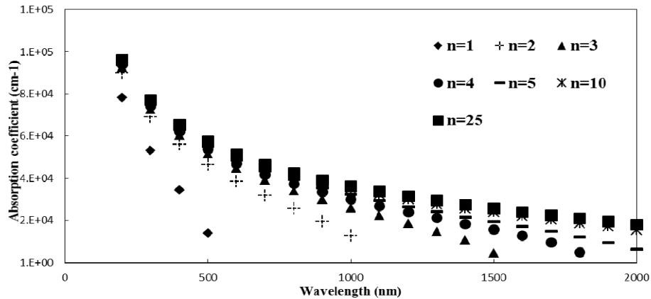
Figure 1 Absorption coefficient of the bP according to wavelength and the number of layers
