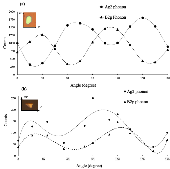
Figure 5 (a) Angular dependency of the A_g^2 and B_{2g} phonons for a 20 nm thick bP layer at 532 nm. (b) Angular dependency of the A_g^2 and B_{2g} phonons for a 10 nm thick bP layer at 532 nm.
