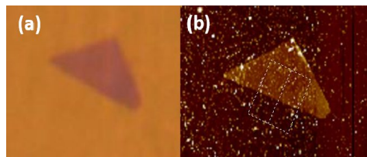
Figure 2 (a) optical image of a bP exfoliated layer (b) AFM measure of the same bP layer: 2-3nm thick
