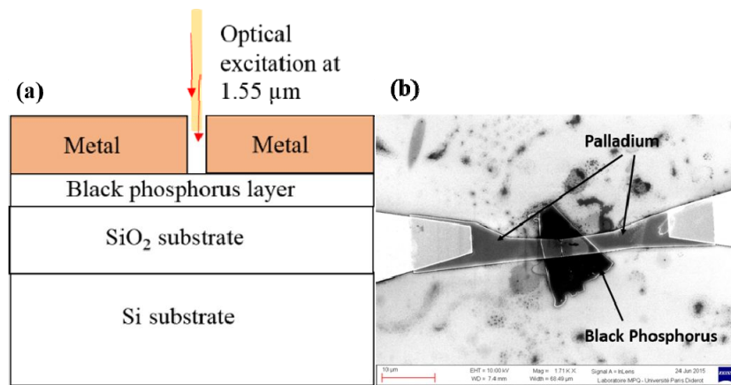
Figure 8 (a) Schematic bP-based photoconductive switch on a Si/SiO 2 substrate. (b) SEM image of a microwave photoconductive switch.
