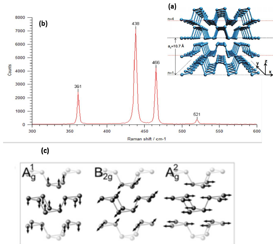
Figure 3 (a) atomic structure of n=4 layer of bP. (b) Typical Raman spectra of the black phosphorus, the 361, 438, 466, 521 peak correspond respectively to A_g^1 , B_{2g} , A_g^2 and the silicium substrate. (c) Three Raman modes in the bP and their vibrations directions.
