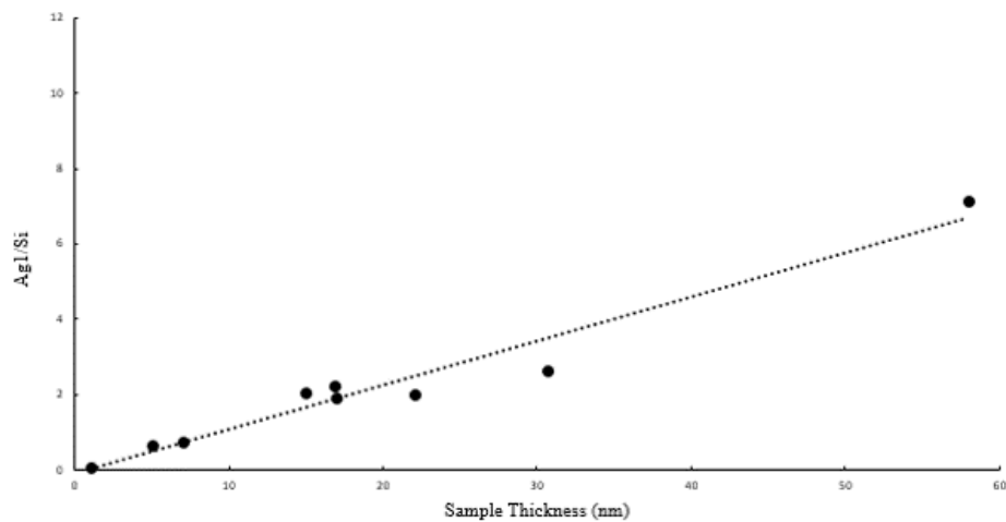
Figure 4 Evolution of the A_g^1 /Silicium Raman intensity with thickness
