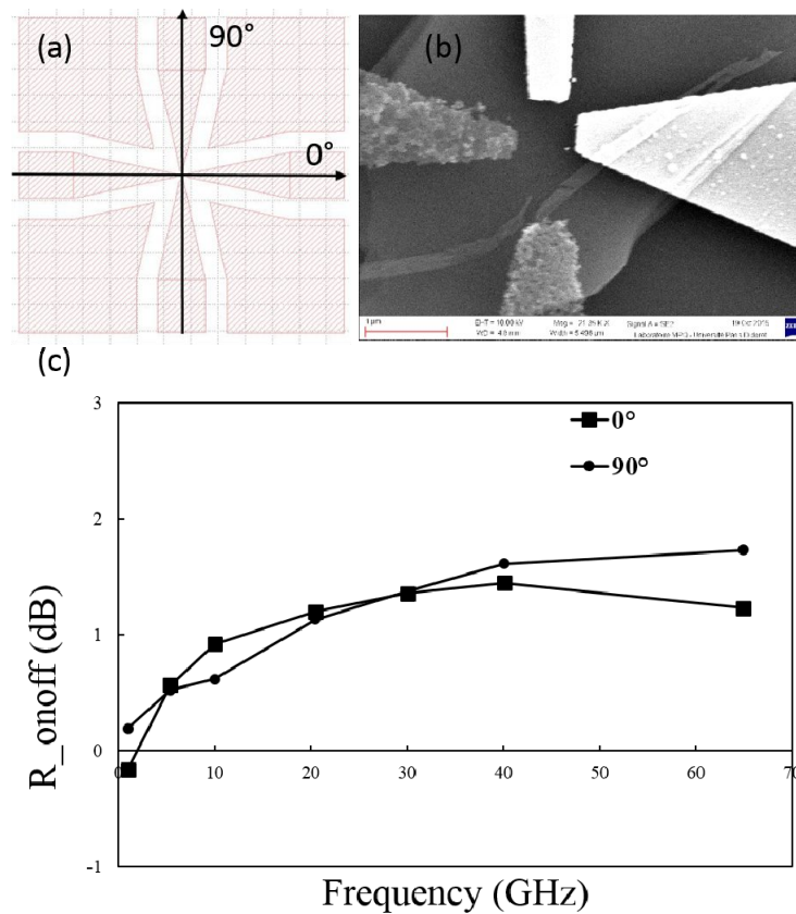
Figure 10 (a) Rectangular microwave photoconductive switch (b) Scanning electron microscopy of the Al/Pd electrodes based on a 50 nm thick bP layer (c) ON/OFF ratio obtained according to the frequency for two directions with 90° between them.
