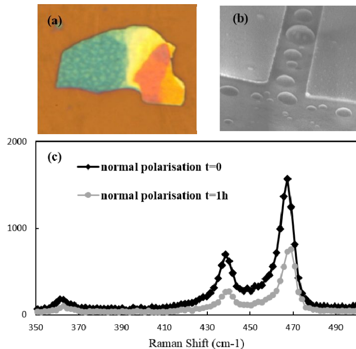
Figure 7 (a) Optical image of exfoliated bP. Observation of droplets at its surface. (b) SEM image of the droplets at the surface of the black phosphorus, and between two electrodes. (c) Raman spectroscopy (532nm, normal polarization) of a 2nm thick bP layer just after exfoliation and one hour after exfoliation.
