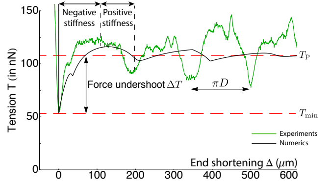
Fig. 3 Drop-on-coilable-fibre systems present an alternance of regimes of positive and negative stiffnesses. Comparison between numerical computations (black line) and experimental data (green line) on a TPU/silicone oil system (drop length 62 \pm 2 \mu\text{m} , TPU fibre diameter 1.9 \pm 0.4 \mu\text{m} and dimensionless capillary force f_\gamma = 41 \pm 20 > f_\gamma^{\text{th}} = \pi^2 , see Section 2.2). The one coil period and the initial negative stiffness regime are well reproduced by the numerical model. Adapted from our previous work in Eletto et al. 21 .
