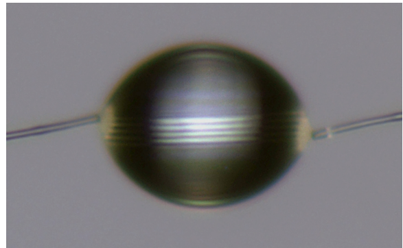
Fig. 1 Thin fibres may buckle and coil inside a liquid drop. A soft thermoplastic PolyUrethane fibre (Young modulus E = 17\text{MPa} ) with radius r = 2.75\mu\text{m} is spooled within a silicone oil drop of diameter D = 191\mu\text{m} 21 .
