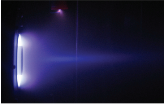
FIGURE 2: ATON A-3 running with krypton.
