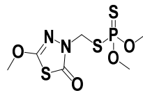
Methidathion log P = 2.5
