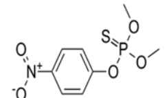
Parathion methyl log P = 3.2
