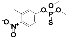
Fenitrothion log P = 3.32
