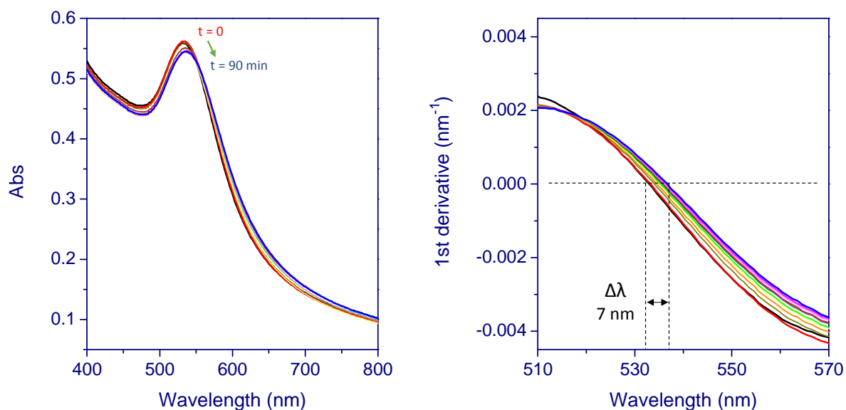
Figure 4. Left: LSPR curves measured upon incubation of AuNP-Ab conjugate with unspiked milk (black trace) and at increasing incubation time (from 0 to 90 min) with 1 \mu\text{g/mL} SEA in milk (red to blue curves). Right: The first derivatives of the LSPR curves.
