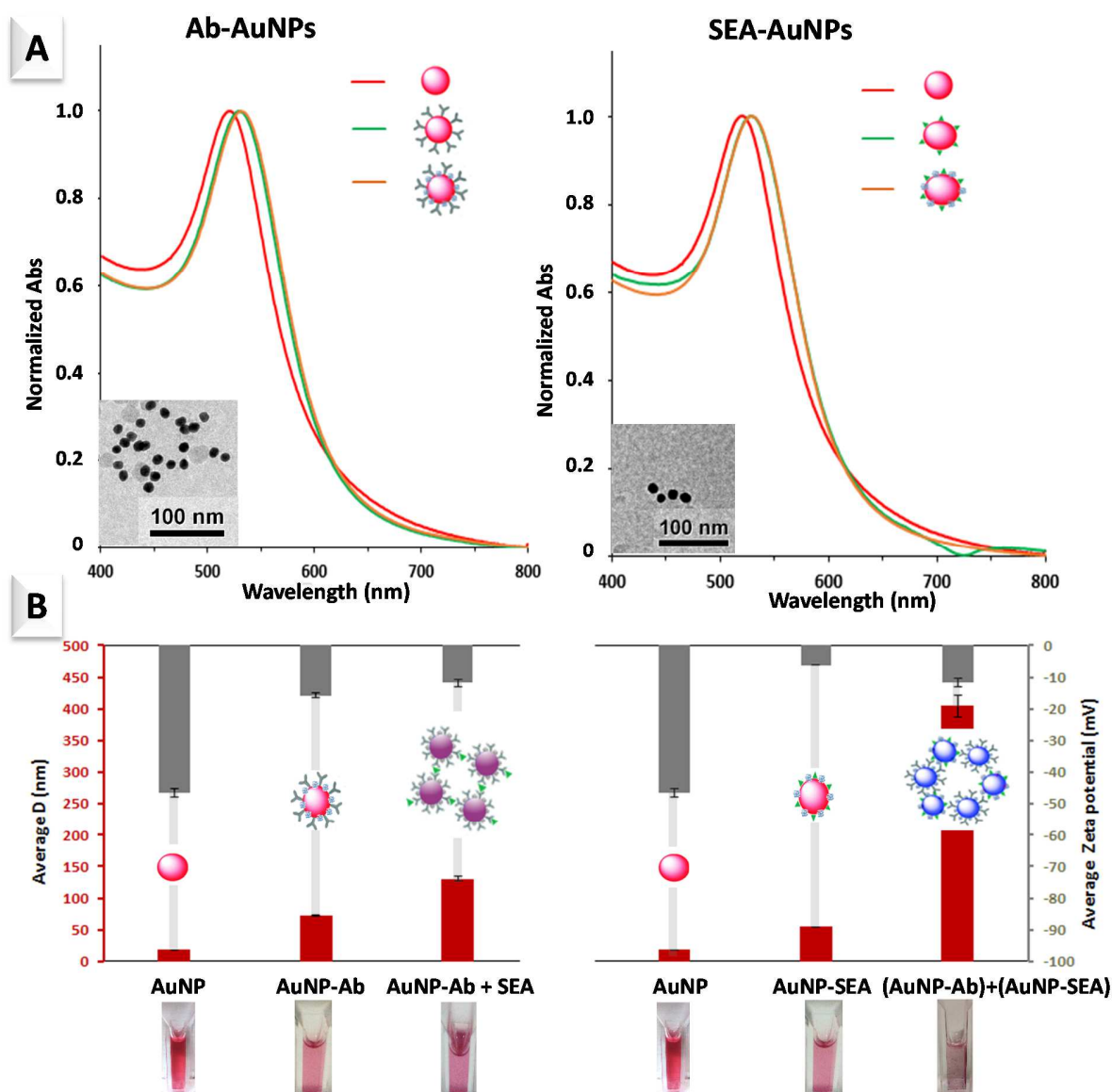
Figure 2 A: LSPR band change upon conjugation of anti-SEA Ab (left) and SEA (right) to AuNPs and subsequent BSA backfilling. The inserts show representative cryo-TEM images of AuNP-Ab and AuNP-SEA bioconjugates. B: hydrodynamic diameter and zeta potential of citrate-coated AuNP, AuNP conjugates and mixtures of AuNP-Ab and free SEA or AuNP-SEA conjugate (5 \mu\text{g/mL} ). Images of the corresponding solutions are added below.
