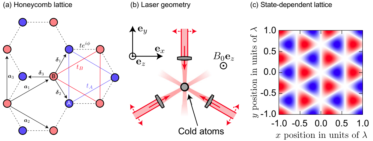
Figure 1. (a) Honeycomb lattice composed of two coupled triangular sublattices A and B. The site positions in each sublattice are defined as \mathbf{r}_{m_A} = m_1\mathbf{a}_1 + m_2\mathbf{a}_2 and \mathbf{r}_{m_B} = m_1\mathbf{a}_1 + m_2\mathbf{a}_2 - \delta_2 , with unit vectors \mathbf{a}_1 = \delta_1 - \delta_3 and \mathbf{a}_2 = \delta_2 - \delta_3 and with m = (m_1, m_2) integer. The NN vectors are \delta_1 = a/2(1, \sqrt{3}) , \delta_2 = a/2(1, -\sqrt{3}) and \delta_3 = a(-1, 0) . We define \mathbf{a}_3 = \mathbf{a}_1 - \mathbf{a}_2 = \delta_1 - \delta_2 . The hopping factors between NN and NNN sites of the honeycomb lattice are indicated by t_A, t_B and te^{i\phi} , with \phi \equiv \phi(m_A, m_B) given by equation (3). The lattice spacing is a\sqrt{3} , and we set a = 1 in the main text, which defines our unit of length. (b) Three-beam laser configuration giving rise to the desired spin-dependent hexagonal lattice, which we describe for ^{40}\text{K} . In this vision, the lasers are detuned between the D1 and D2 lines of the 4S–4P transition, whereby the state-independent (scalar) light shift is zero. The remaining spin-dependent potential—an effective Zeeman magnetic field—is depicted in (c). The strength of the ‘same-spin’ hopping, i.e. t_a and t_b , is governed by the choice of internal states: the pair |f = 9/2, m_F = 7/2\rangle and |f = 7/2, m_F = 7/2\rangle produce t_a \approx t_b as they have opposite magnetic moments. In contrast, the choice |f = 9/2, m_F = 9/2\rangle and |f = 7/2, m_F = 7/2\rangle produces t_a \neq t_b . The effective Zeeman shift is plotted with a color scale where blue indicates the potential minima for pseudo-spin up atoms, forming the A sublattice; and red indicates the minima for pseudo-spin down atoms, forming the B sublattice. Not shown are an additional pair of Raman lasers, also in the \mathbf{e}_x - \mathbf{e}_y plane, that couple between the different sublattices (red and blue in (c)).
