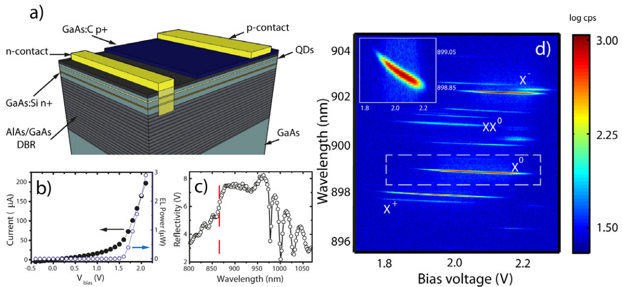
Figure 3. (a) Device structure. In order to control the charge of the QDs, an n-doped GaAs layer below, together with a p-doped GaAs layer above the actual QD layer, forms a p–i–n diode structure. An additional AlGaAs blocking barrier between the QD layer and the p-doped region prevents excessive current flow. (b) The I – V characteristic (black) for the p–i–n diode and electroluminescence signal (blue) as a function of the applied gate voltage at low temperature. (c) Measured reflectivity of the semiconductor DBR mirror between 800 and 1050 nm. The vertical dashed red line indicates the GaAs bandgap energy. A minimum in reflectivity around 940 nm arises from a systematic measurement error. (d) QD charging plateaus. PL signal (logarithmic scale) as a function of gate voltage and wavelength. The different voltage regions corresponding to the different charging plateaus of the same QD are clearly visible. The inset shows a blow-up of the X^0 plateau, with the quantum-confined Stark effect leading to a significant tilt in the plateau as a function of gate voltage. Note that for the measurement results shown here the sample was characterized in a flow cryostat leading to higher temperature, i.e. higher resistivity, and therefore to a higher voltage range than in part (b).
