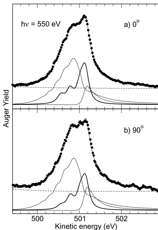
Figure 5. The Auger spectrum in the energy region from 499.4 to 502.9 eV subsequent to an ionization with 550 eV photons measured at an angle of (a) 0° and (b) 90° relative to the polarization of the light. The solid line through the data points represents the fit result. The thin solid subspectra represent the O 1s^{-1} \rightarrow a^1\Sigma^+ and O 1s^{-1} \rightarrow b^1\Pi normal Auger transitions, the bold solid subspectrum the resonant Auger transitions and the dashed subspectrum the background.
