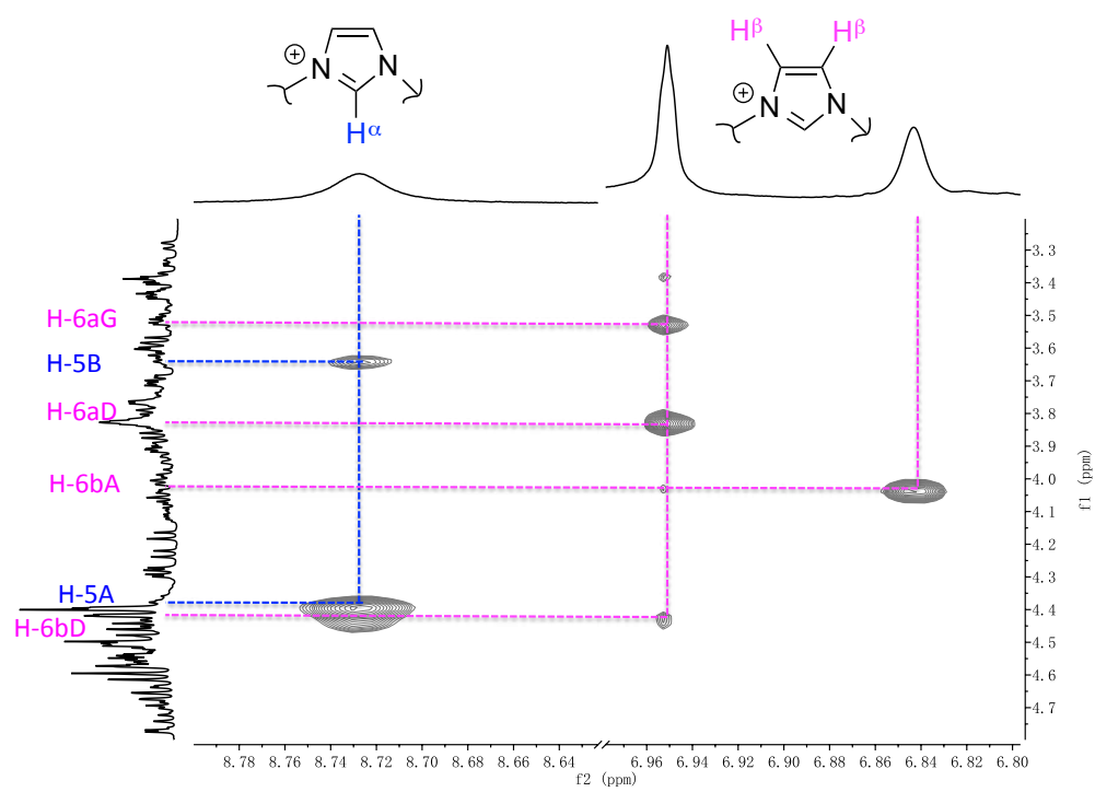
Figure S4. Key NOESY cross peaks of imidazolium ( \gamma -A,D-ICyD)HCl, CD 3 CN, 600 MHz, 300 K
