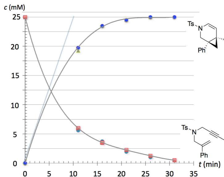
Figure S19. Cycloisomerization catalyzed by (IPr)AuCl at 300K in \text{CD}_2\text{Cl}_2 . Plot of the concentrations as a function of time. The slope at c = 0 for the cyclized product (blue line) gives an initial rate r_0 of ca. 41.6 \cdot 10^{-6} \text{ mol L}^{-1} \text{ s}^{-1} .
