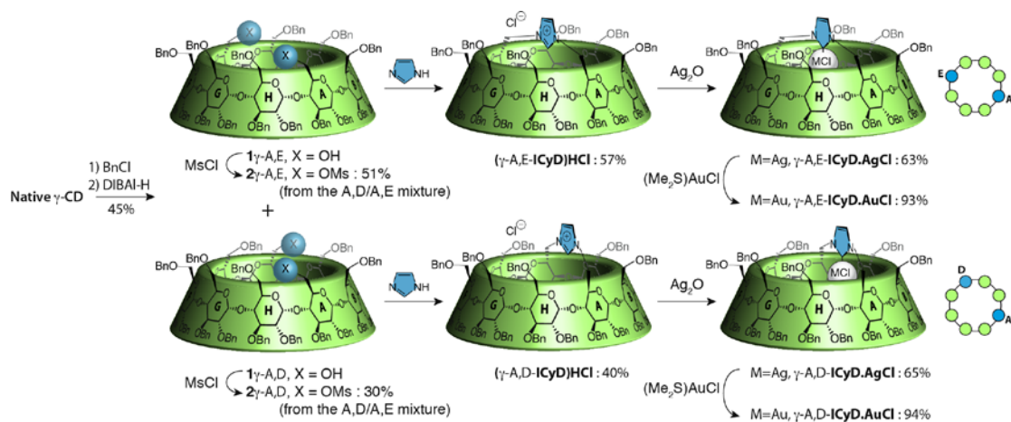
Scheme S2. Synthesis of \gamma -A,E- and \gamma -A,D-ICyD silver and gold complexes.
